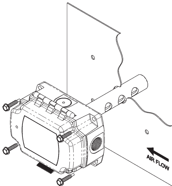
Fig. 2: Duct unit mounting
