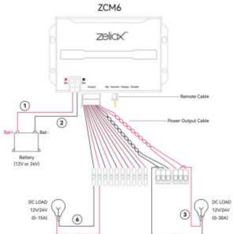
Figure 3-2 Single ZCM6 wiring
