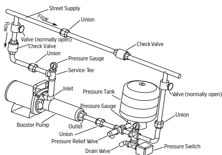
Pump Installation Using Municipal Source
