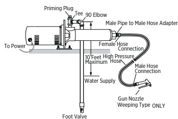
Pump Installation Drawing Water from Below Pump
