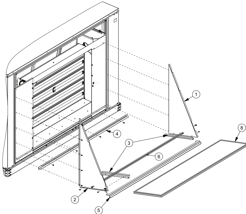
Figure 19. Hood assembly
