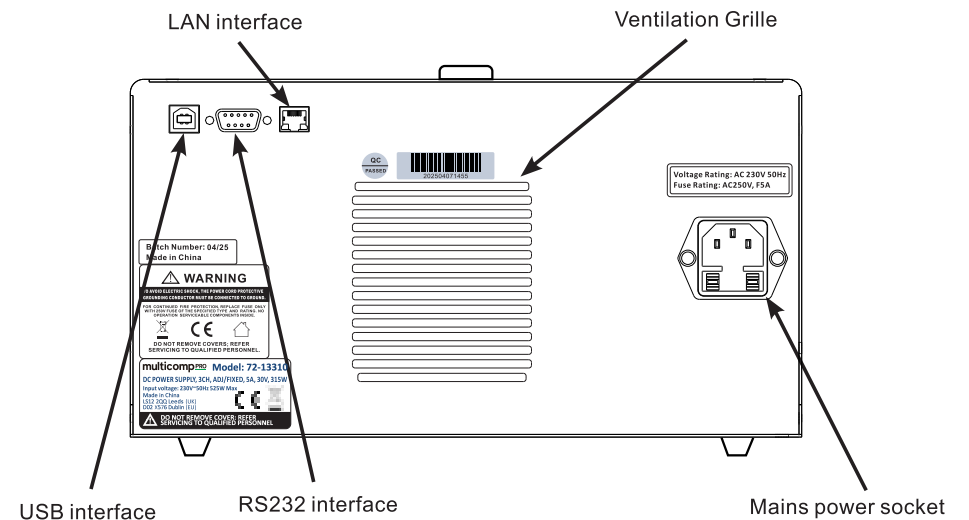
Rear Panel
