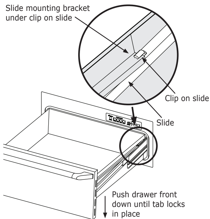
Drawer Installation
