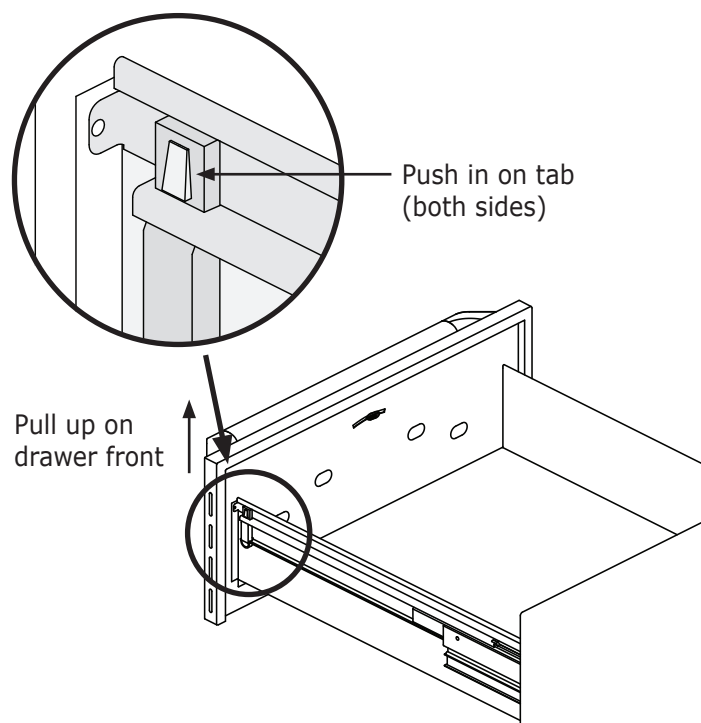
Drawer Removal
