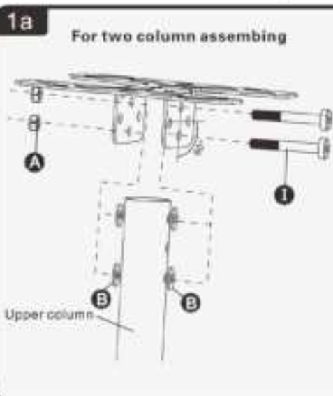
Ceiling Mount For medium TVs and displays For screen sizes 32"-65" Weight capacity: 35kg / 77 lbs VESA: 100x100-600x400
