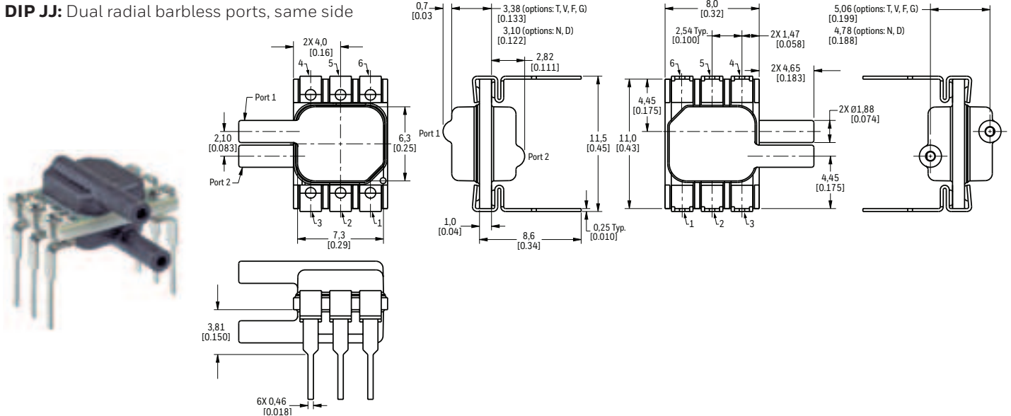
FIGURE 2. DIP PACKAGE DIMENSIONAL DRAWINGS (CONTINUED)
