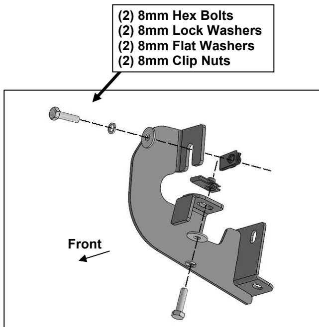
(Fig 3) Attach (1) Passenger/Right Mounting Bracket to the Clip Nuts
