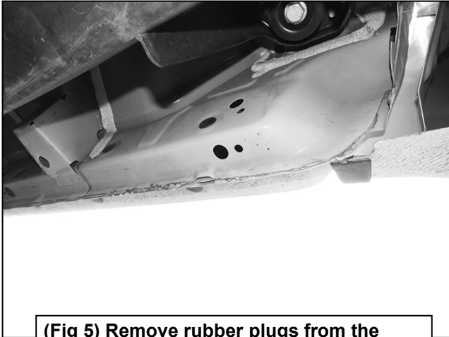
(Fig 5) Remove rubber plugs from the Passenger/Right rear mounting location
