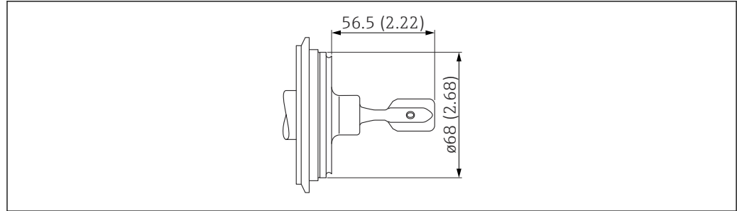
29 Varivent N pipe DN65-162 PN25. Unit of measurement mm (in)
