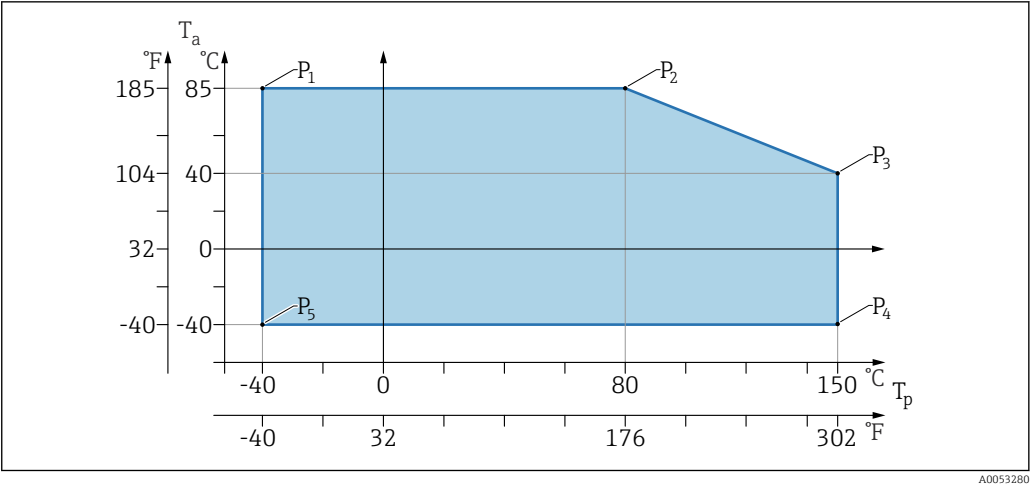
14 Ambient temperature T_a depending on the process temperature T_p
