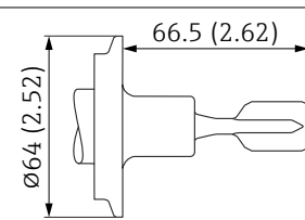
31 Tri-Clamp 2". Unit of measurement mm (in)
