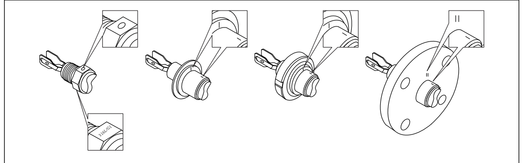
9 Position of the tuning fork when installed horizontally in the vessel using the marking
