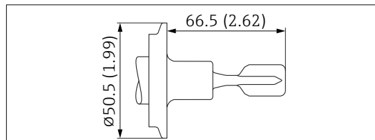
30 Tri-Clamp 1 to 1 1/2". Unit of measurement mm (in)
