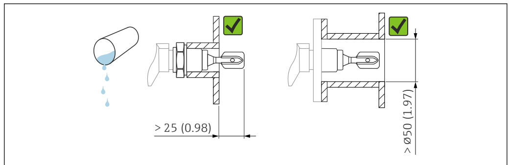
5 Installation example for low-viscosity liquids. Unit of measurement mm (in)
