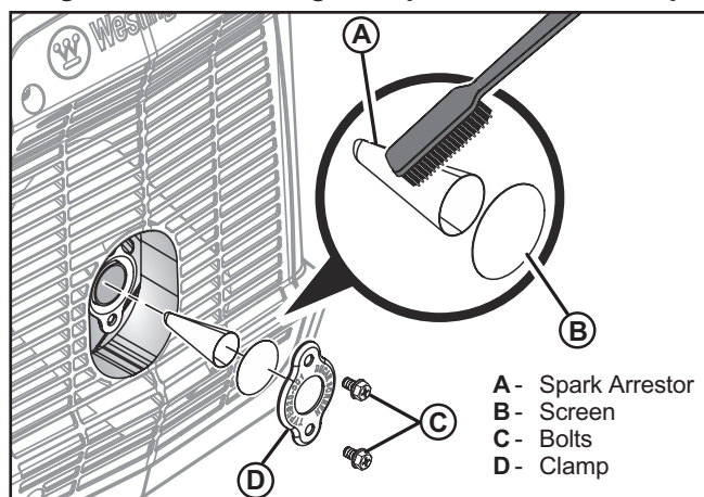
Figure 37 - Removing and Cleaning the Spark Arrestor
