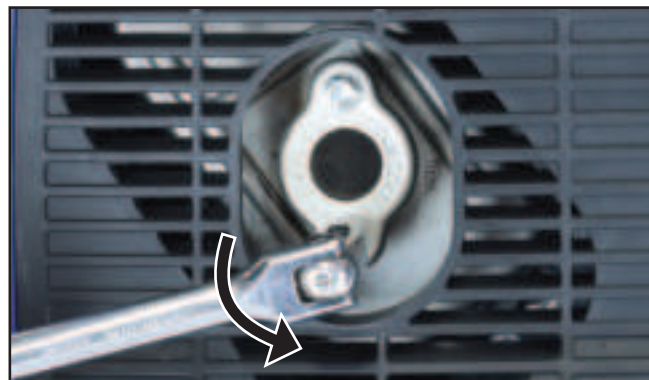
Figure 36 - Removing the Spark Arrestor Clamp
