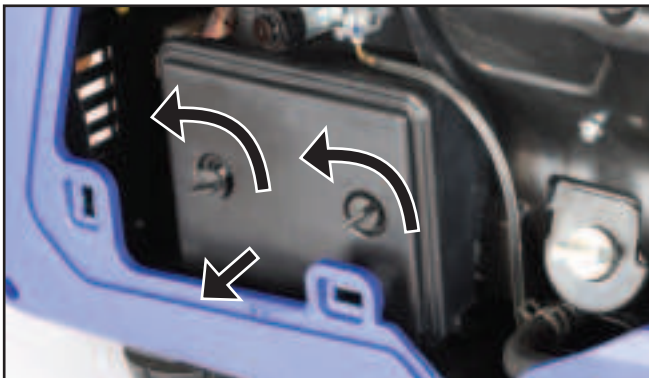
Figure 26 - Removing the Air Filter Cover
