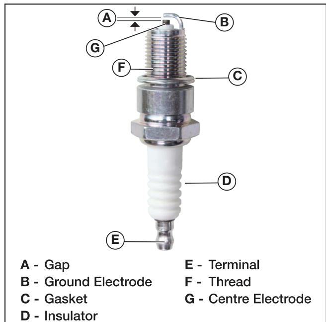
Figure 35 – Spark Plug
