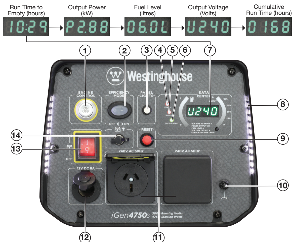
Figure 4 - iGen4750s Control Panel Features
