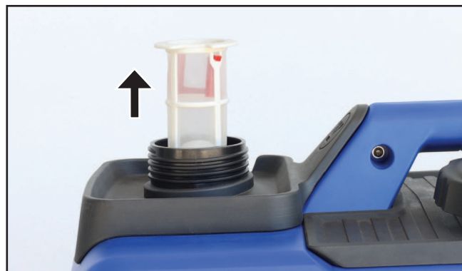
Figure 30 – Removing the Fuel Strainer
