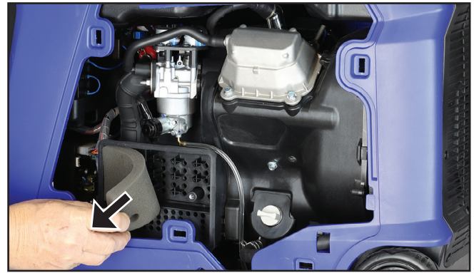
Figure 27 - Removing the Air Filter Element
