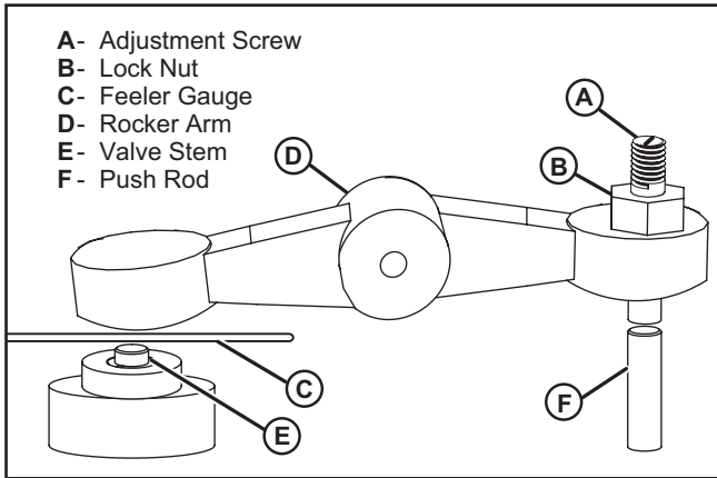
Figure 41 – Adjusting the Valve Clearance
