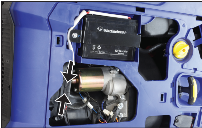
Figure 8 – Assembling the Battery Wiring Harness Connector
