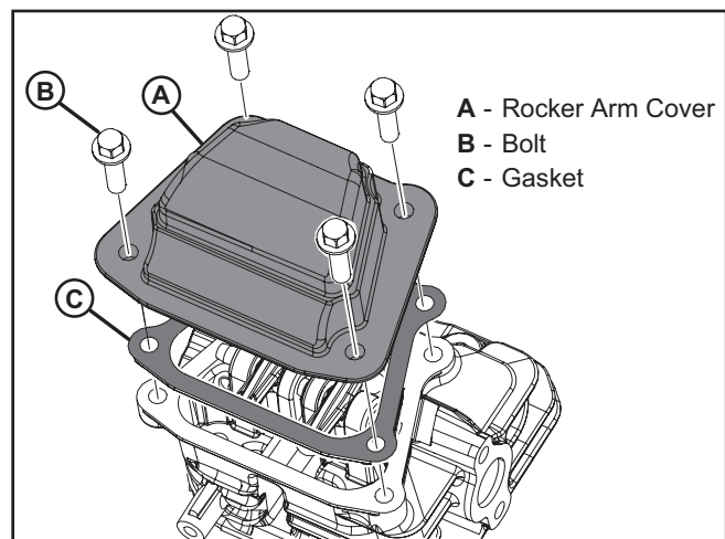
Figure 40 – Removing the Rocker Arm Cover
