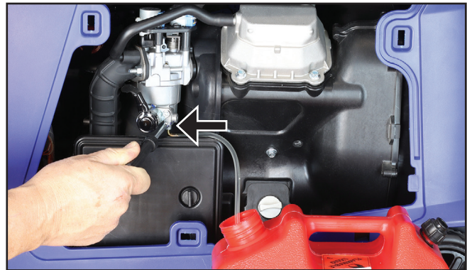
Figure 46 – Draining the Carburettor
