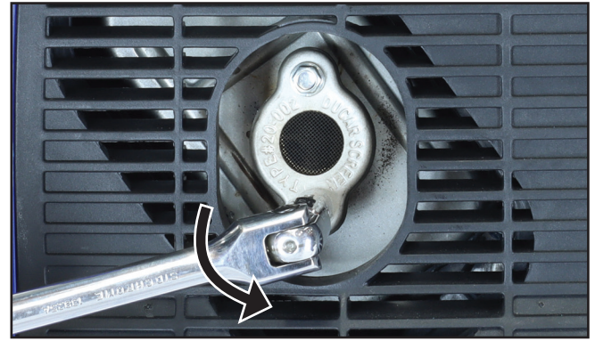
Figure 36 - Removing the Spark Arrestor Clamp
