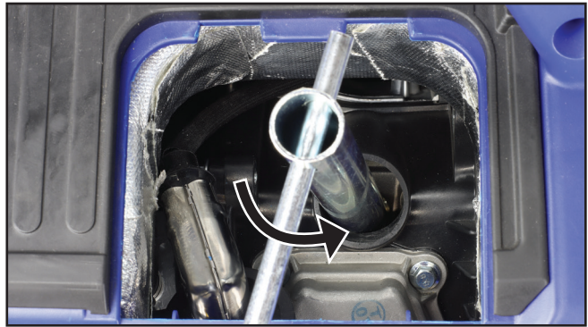
Figure 34 – Removing the Spark Plug
