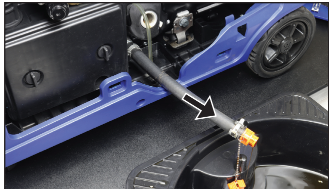
Figure 25 – Draining the Engine Oil
