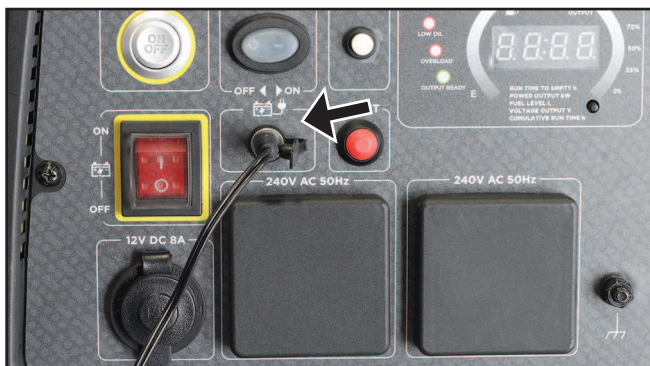
Figure 28 – Connecting the Battery Charger to the Generator
