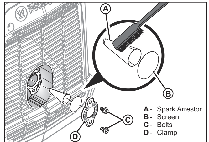
Figure 37 - Removing and Cleaning the Spark Arrestor
