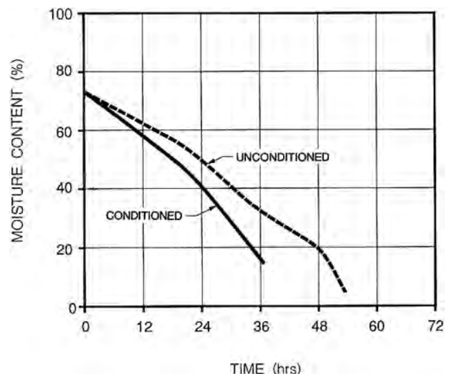
FIGURE 2. The Effect of Conditioning in Alfalfa at 1.2 ton/ac (2.6 t/ha) for the Case IH 8380.
