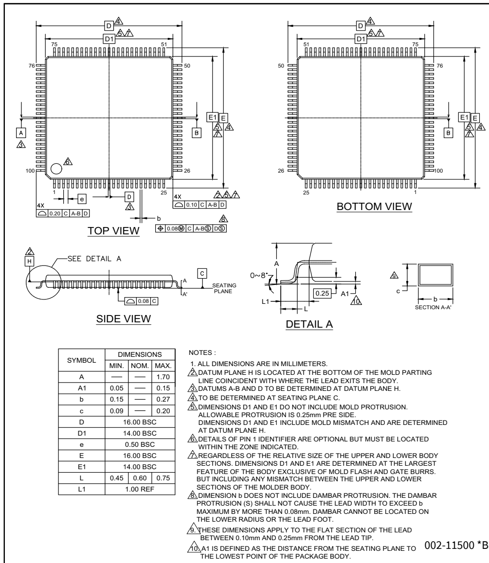
Figure 29-1 100-LQFP package outline
