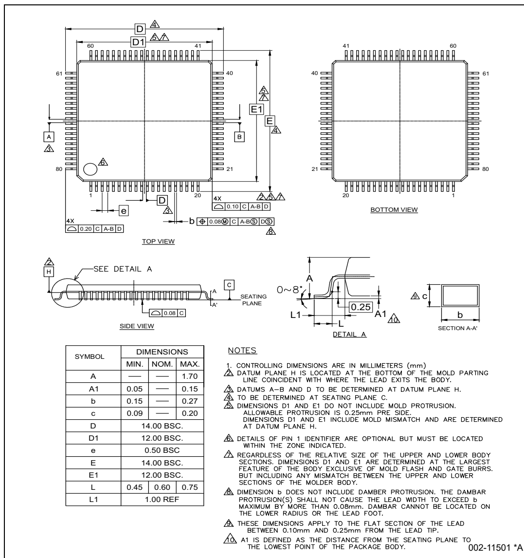
Figure 29-2 80-LQFP package outline
