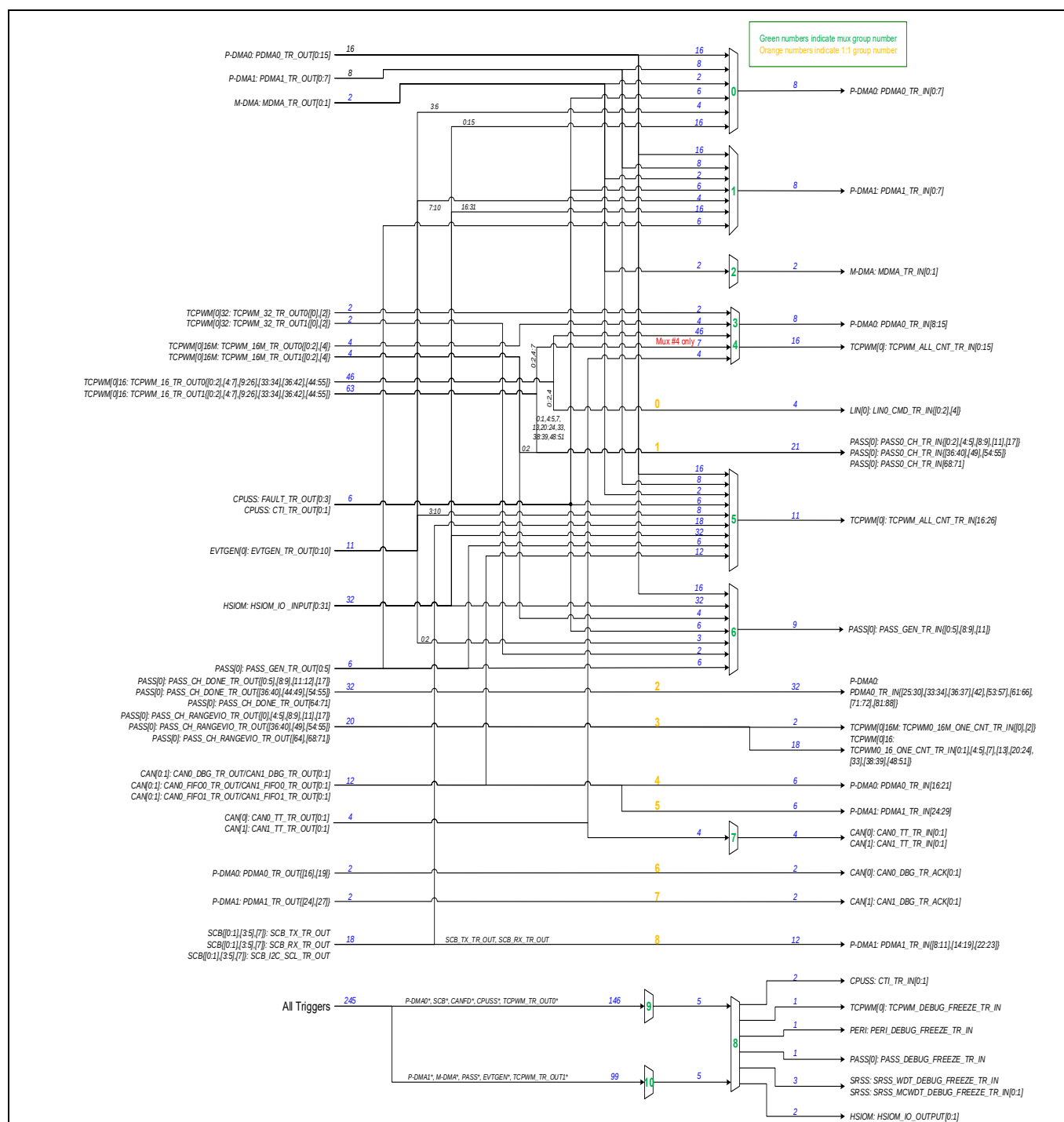
Figure 17-1 Trigger multiplexer [30]
