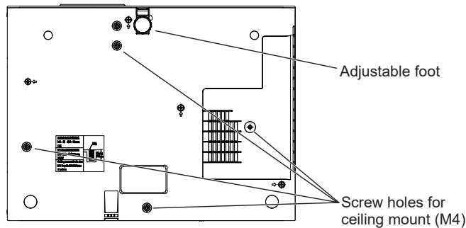
Positions of screw holes for ceiling mount and adjustable foot
