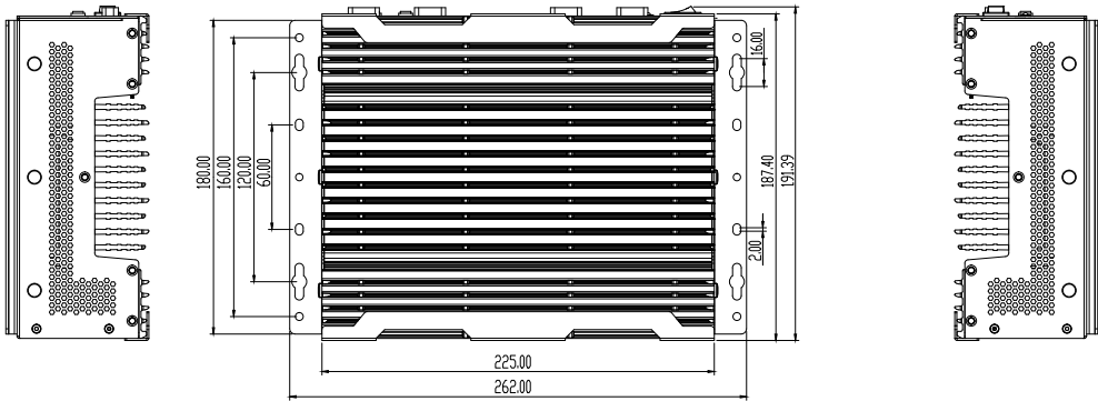
Left View
