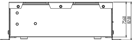
Rear View
