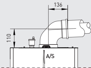
Concentric kit dimensions Ø 80/125*
