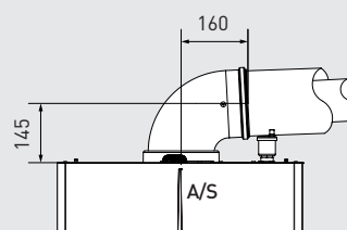
Concentric kit dimensions 110/160*
