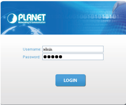
Figure 4-2: Login Screen
