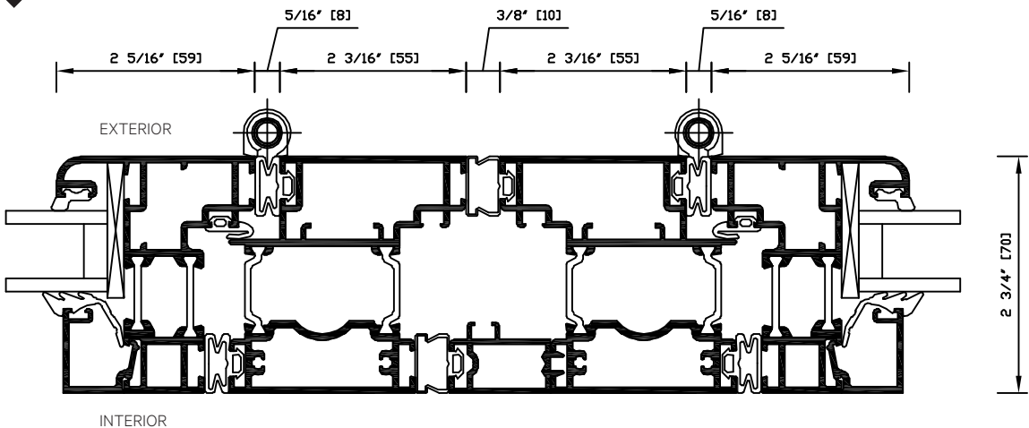
Detail 9R.1 Meeting of panels folding to opposite sides (no swing panel). Running carriage sets on both panels.
