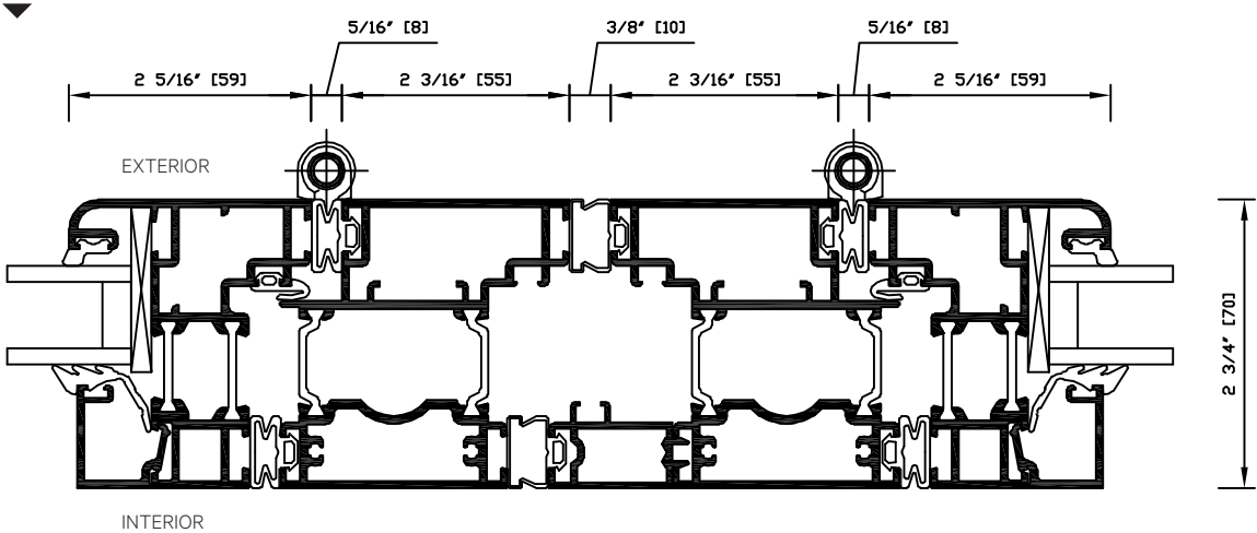
Detail 9R.1 Meeting of panels folding to opposite sides (no swing panel). Running carriage sets on both panels.
