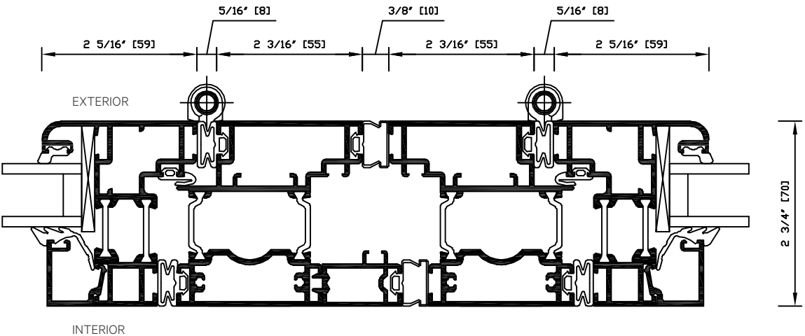
Detail 9.1 Meeting of panels folding to opposite sides (no swing panel). Running carriage sets on both panels.
