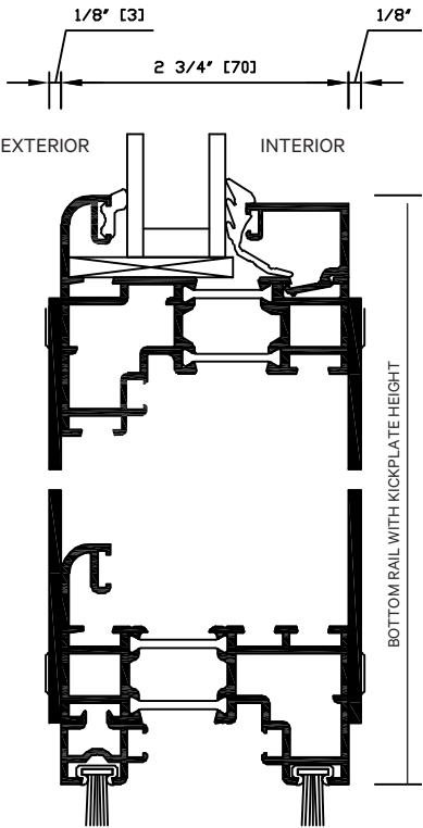
Typical Kickplate
