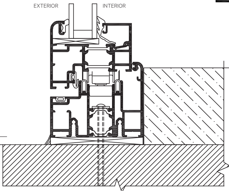
Higher Weather Performance Sill (Raised Sill) Installation
