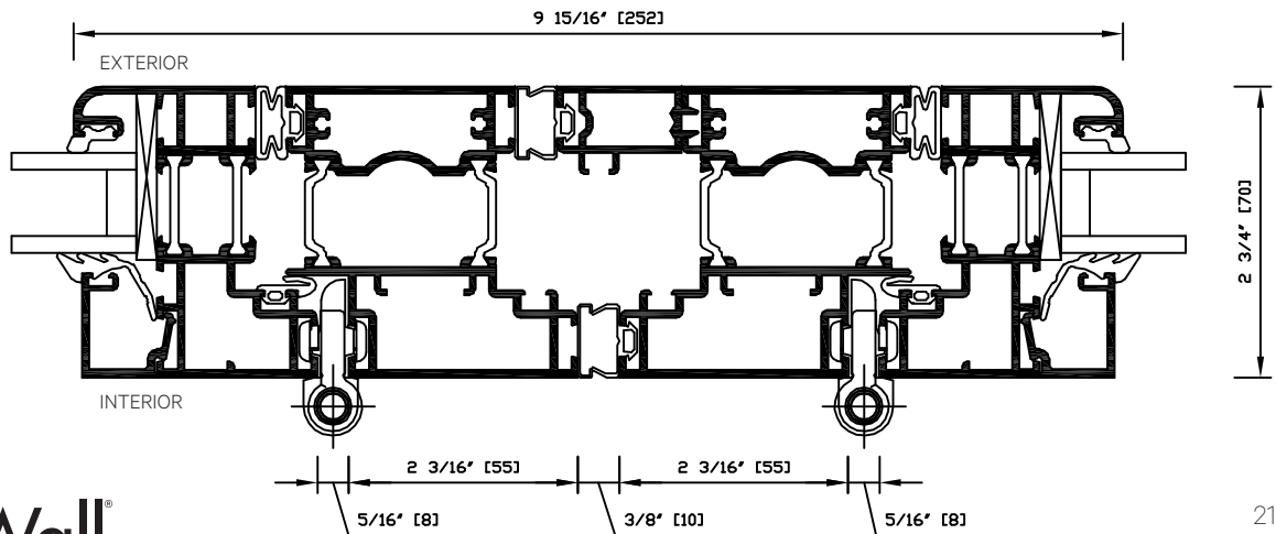
Detail 9.0 Meeting of panels folding to opposite sides (no swing panel). Running carriage sets on both panels
