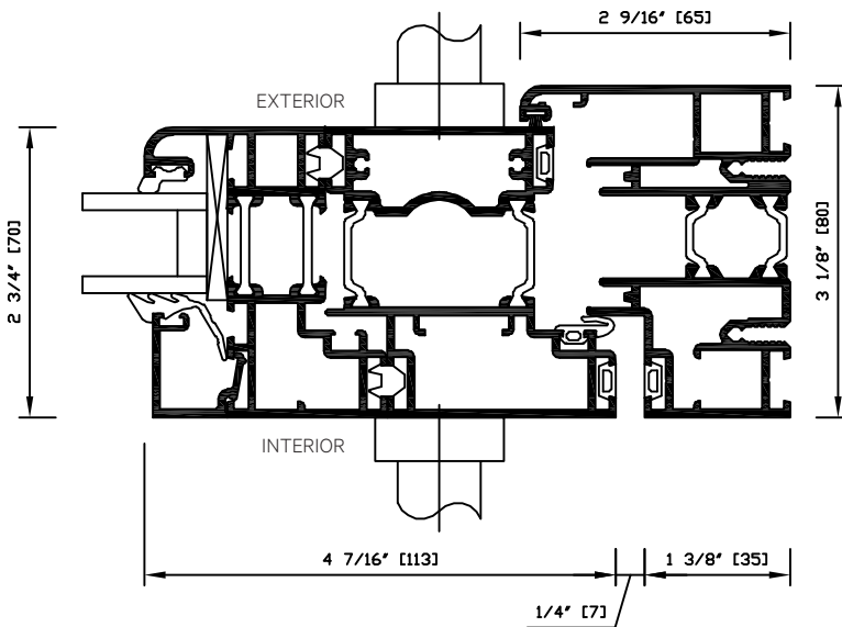
Detail 4R.0 Swing panel with locking right side jamb
