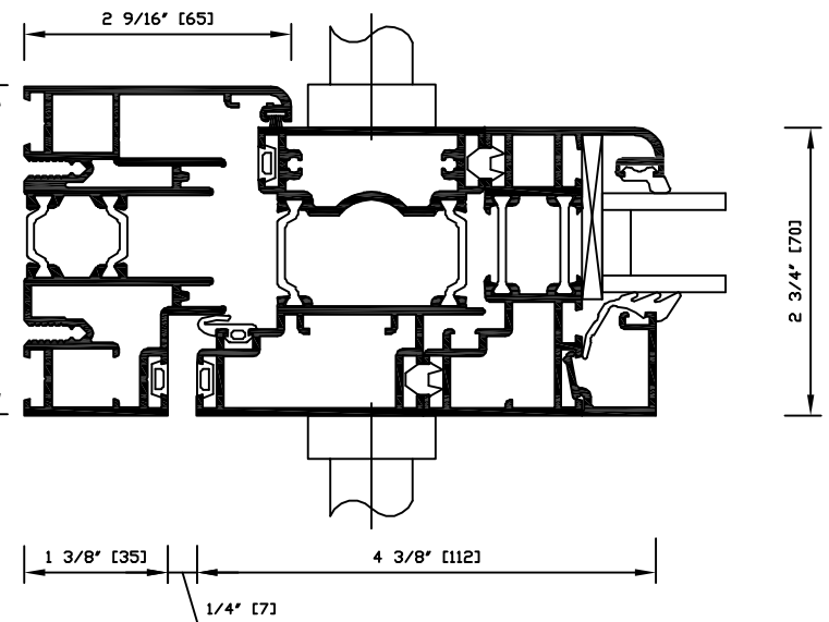
Detail 4.0 Swing panel with locking left side jamb
