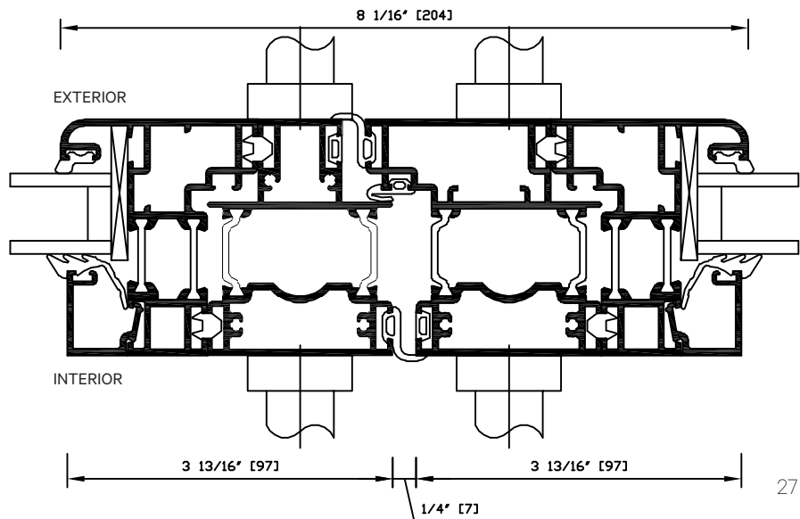
Detail 8R.1 ▶ Two swing panels with locking: right panel opening first
