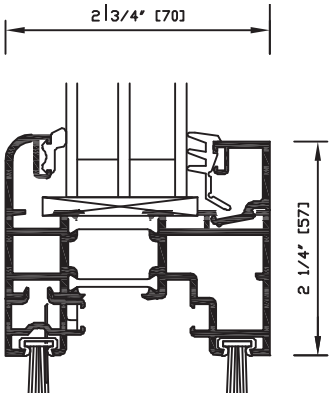
Typical Glass Stop Profile with Triple Glazing
