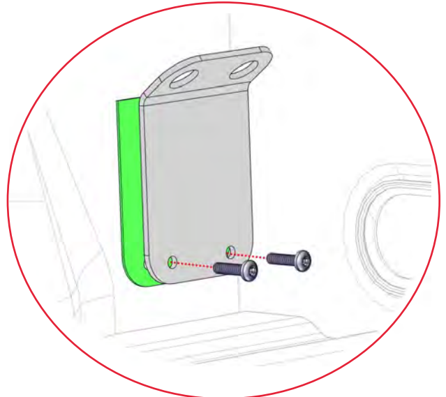
DETAIL B: Install DECKED cabside bracket
