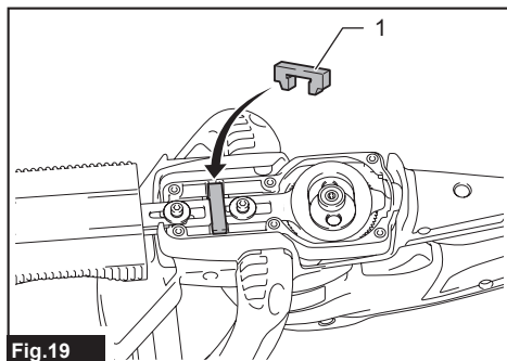
► 1. Felt pad
