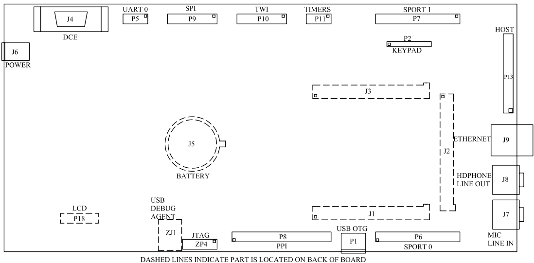
Figure 2-5. Connector Locations
