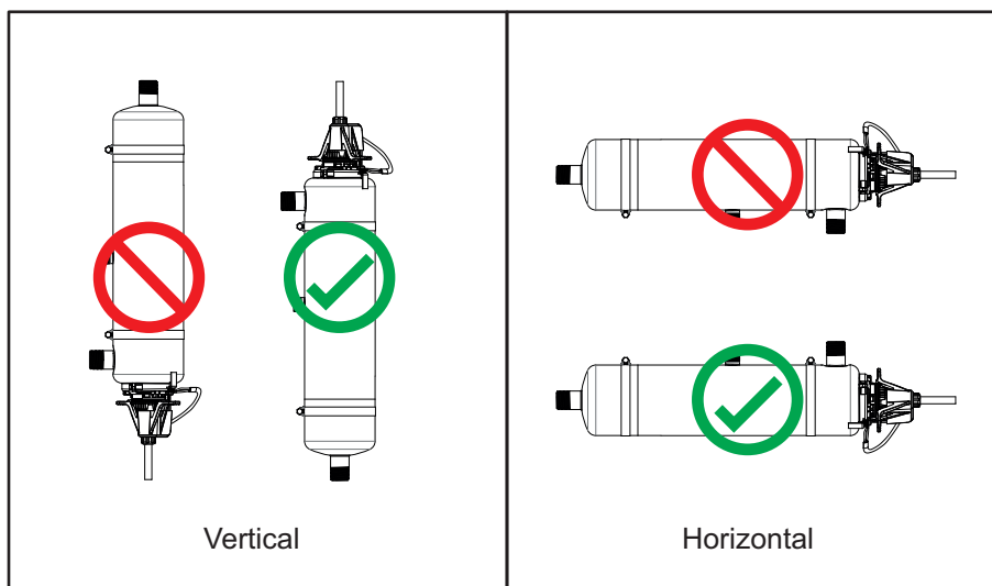
Figure 4 UV System Installation - Vertical and Horizontal
