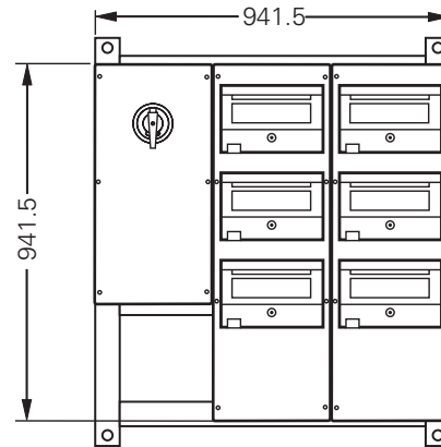
Type 3 X = fixing dimension
