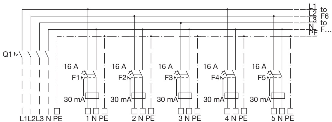
Heating circuits
