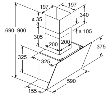
Appliance in exhaust air mode
