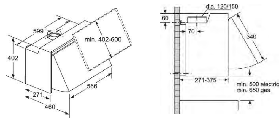
Integrated hoods LE66MAC00B
