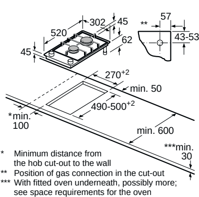
Domino gas hob ER3A6BI40
