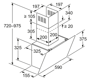
Appliance in circulated air mode
