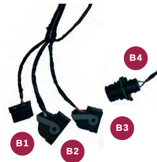
Figure 7 - Terminations of the connection harness
