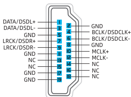
IIS OVER HDMI(Socket view)
