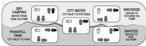
Valve Operation Diagram
