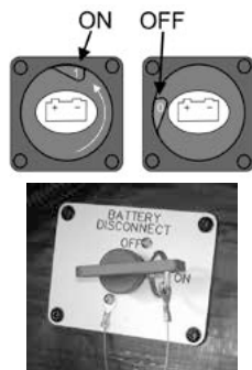
Battery Disconnect Switches
