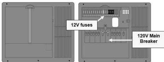
Typical Load Center Panel
