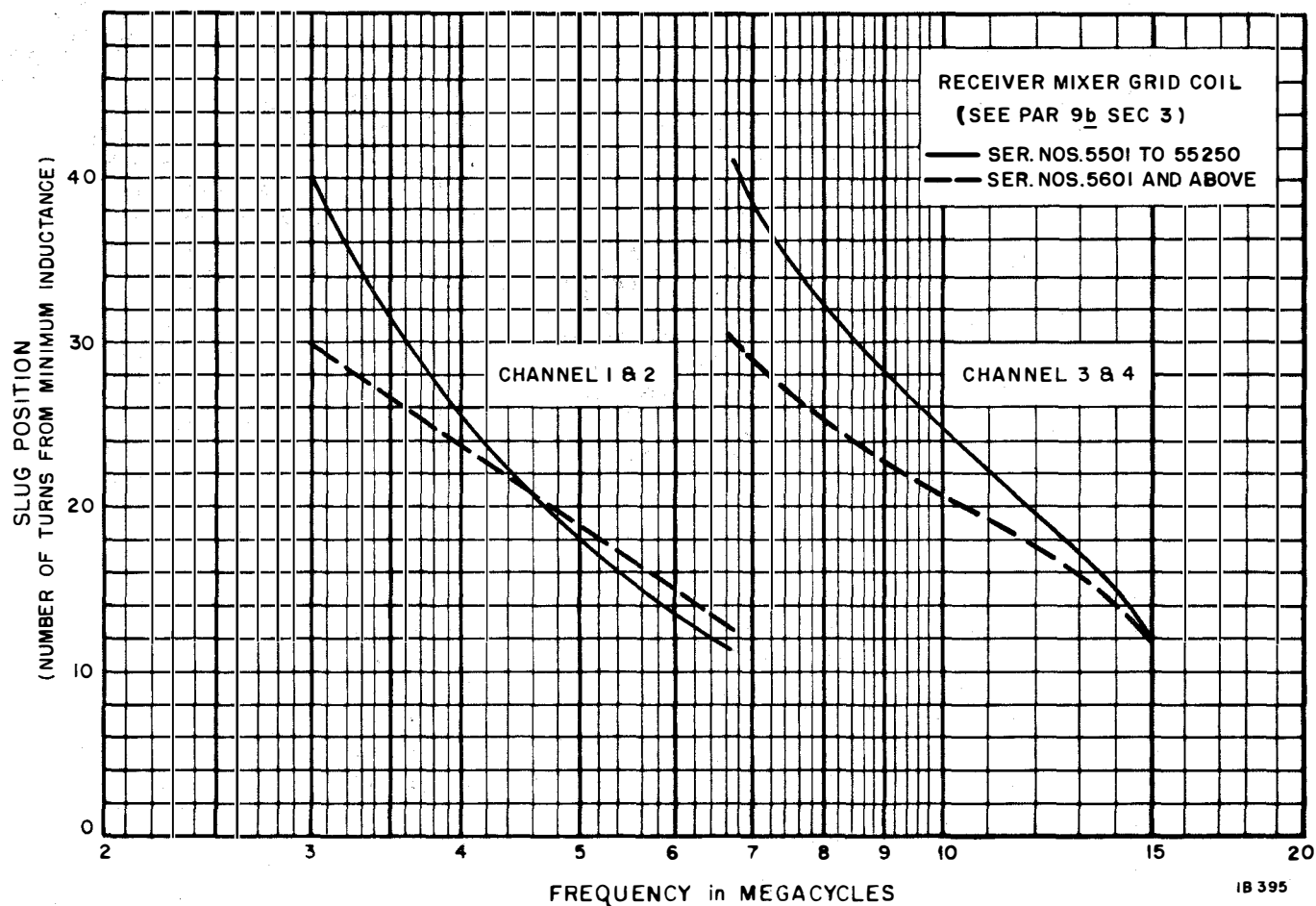
Figure 27. Slug Position of Receiver Mixer Grid Coils
