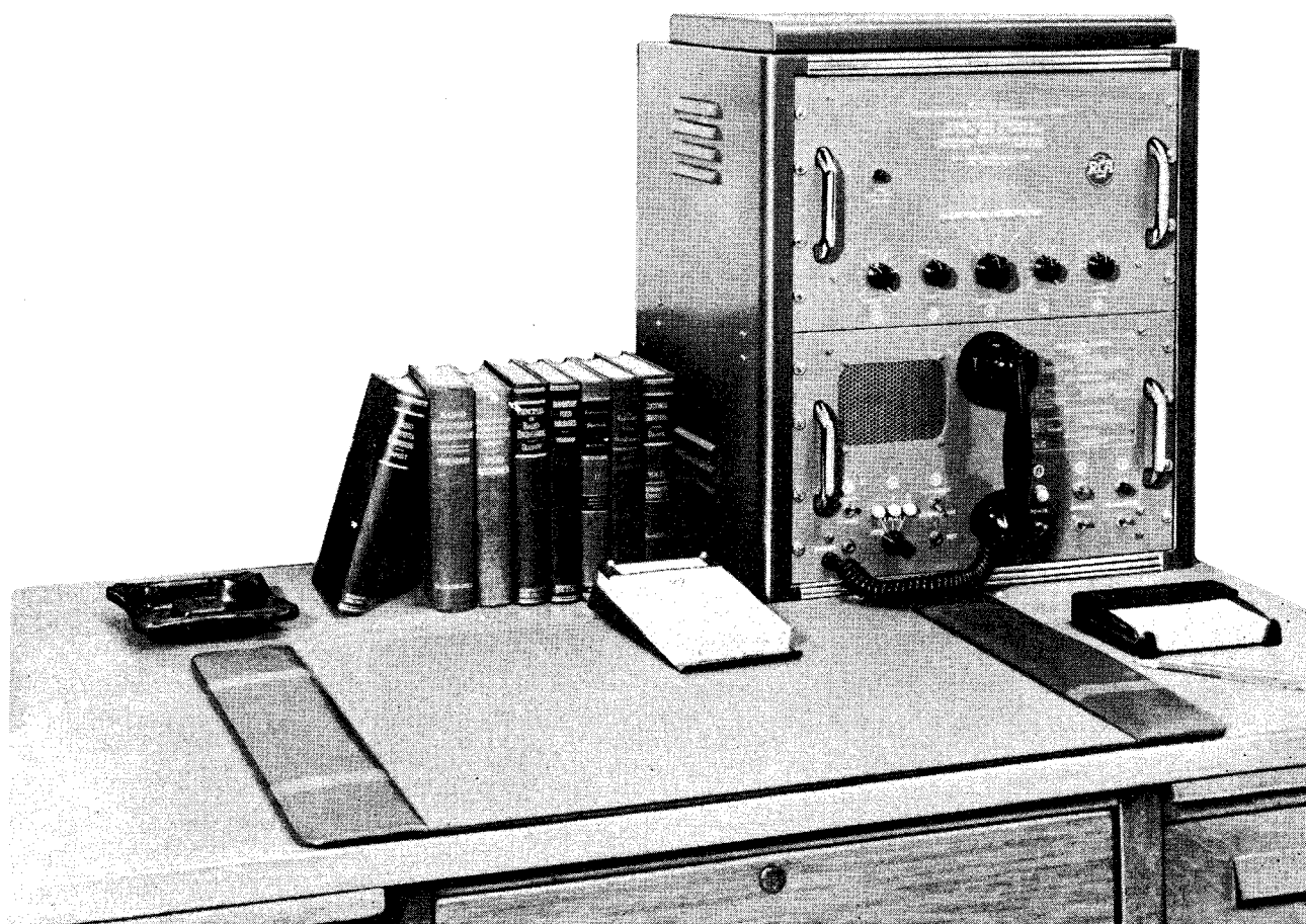
Figure 1. Desk Installation
