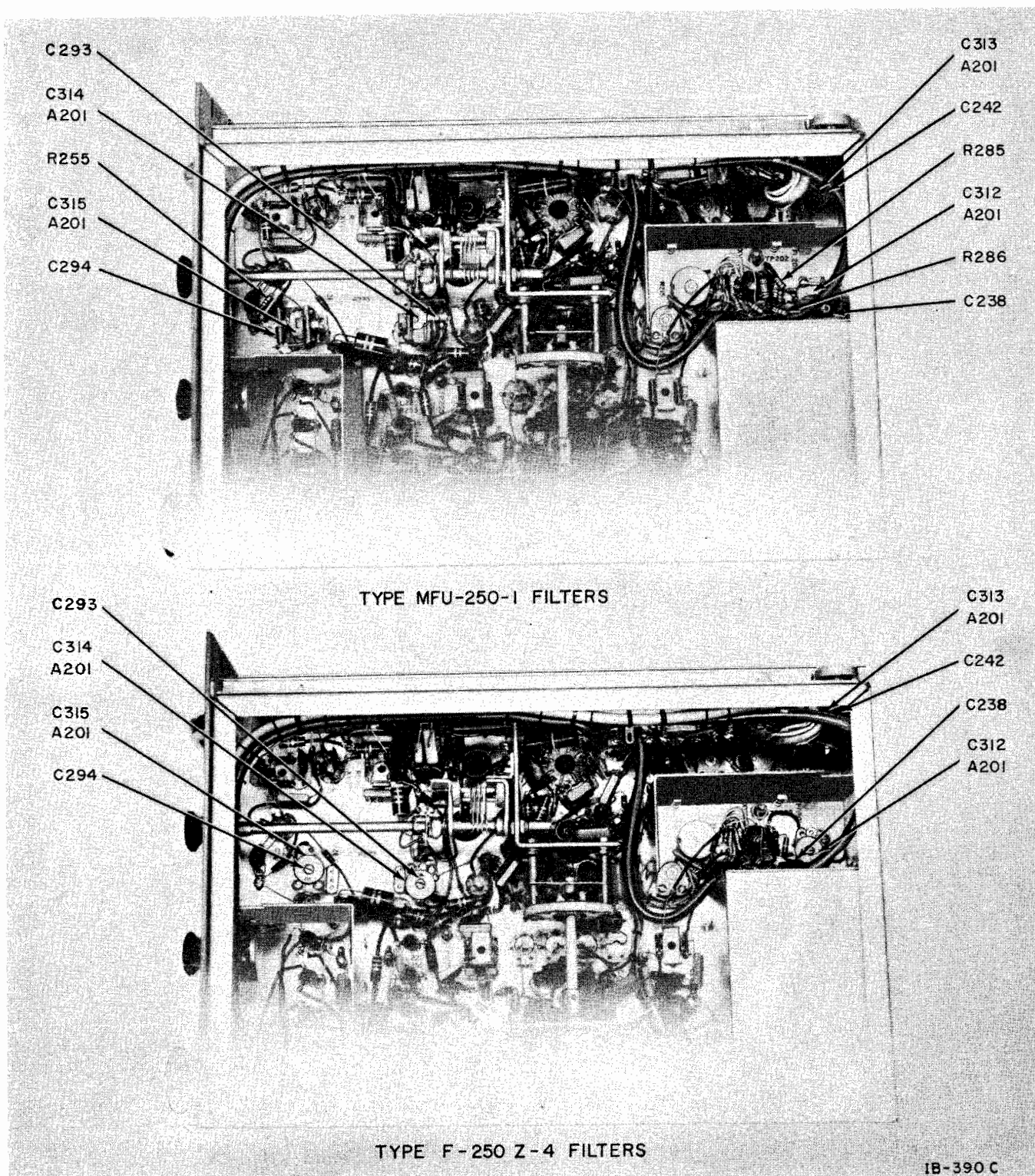
Figure 21C. Transmitter-Receiver, Components Used with Mechanical Filters, Equipments Serial Nos. 5601 and above
