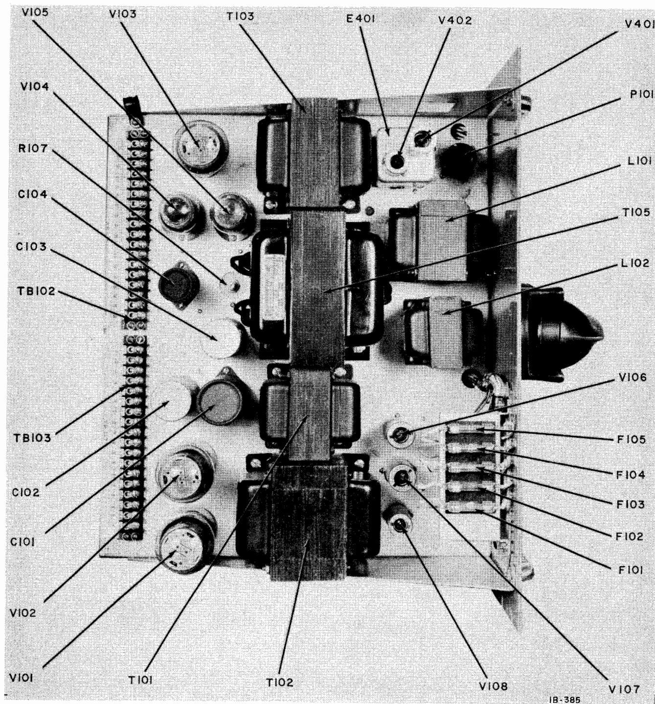
Figure 16. Power Supply, Top View
