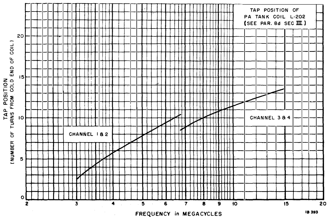
Figure 25. Tap Positions of Plate Tank Coil L-202
