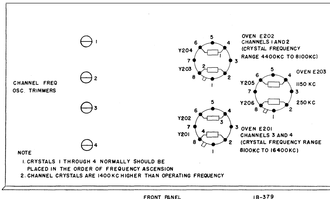
Figure 9. Crystal Ovens, Top View, Cover Removed
