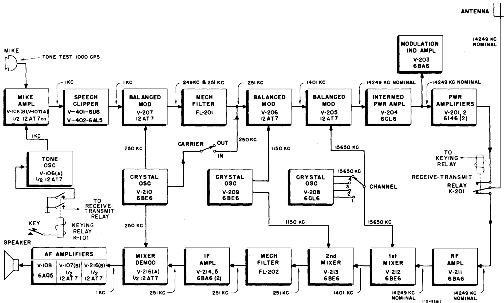
Figure 5. Block Diagram
