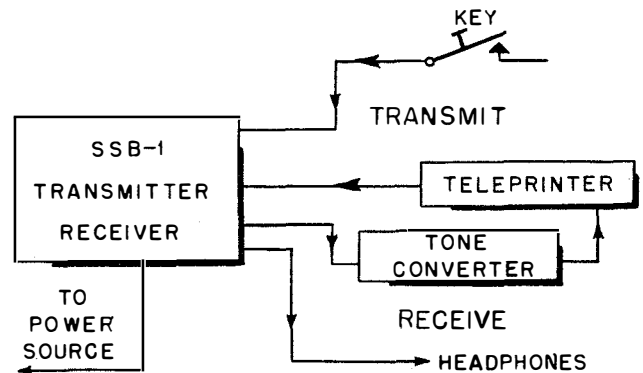
Figure 12. Telegraph and Teleprinter Operation
