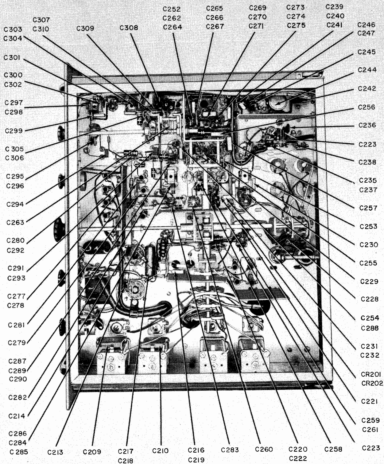
Figure 21A. Transmitter-Receiver, Bottom View, Location of Capacitors
