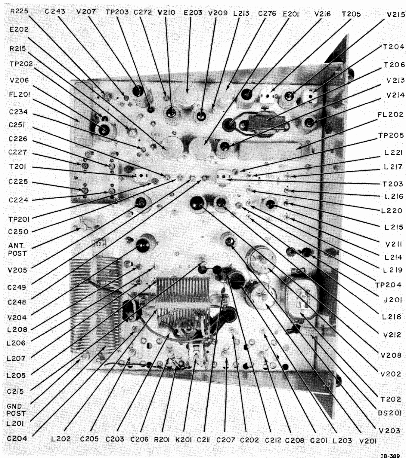
Figure 20. Transmitter-Receiver, Top View
