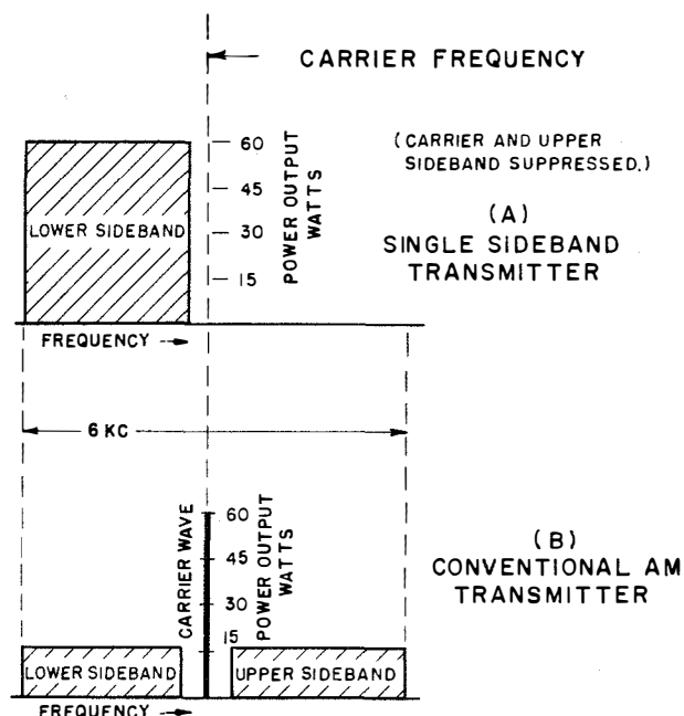
Figure 2. Comparative Frequency and Power of Type SSB-1 and Equivalent AM System
