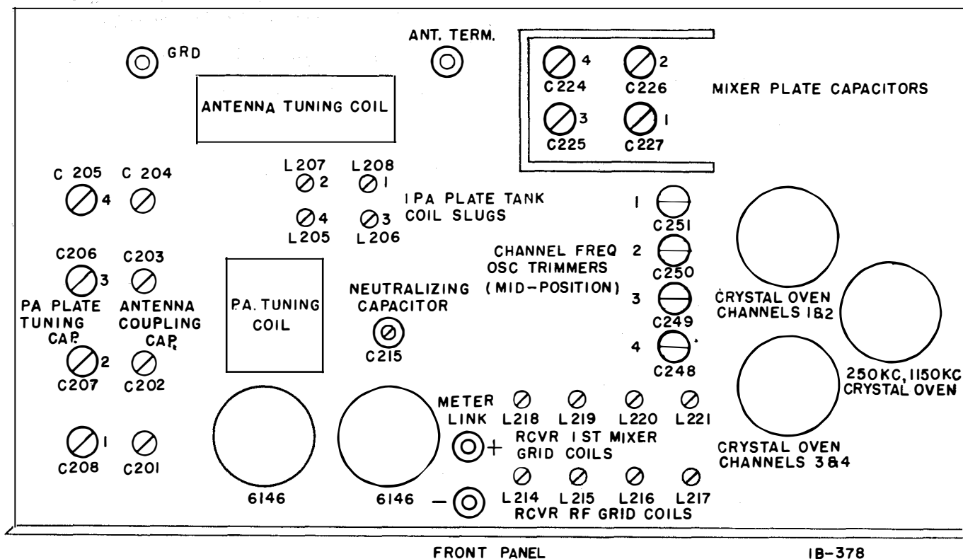
Figure 8. Location of Channel Alignment Components on Transmitter-Receiver Chassis
