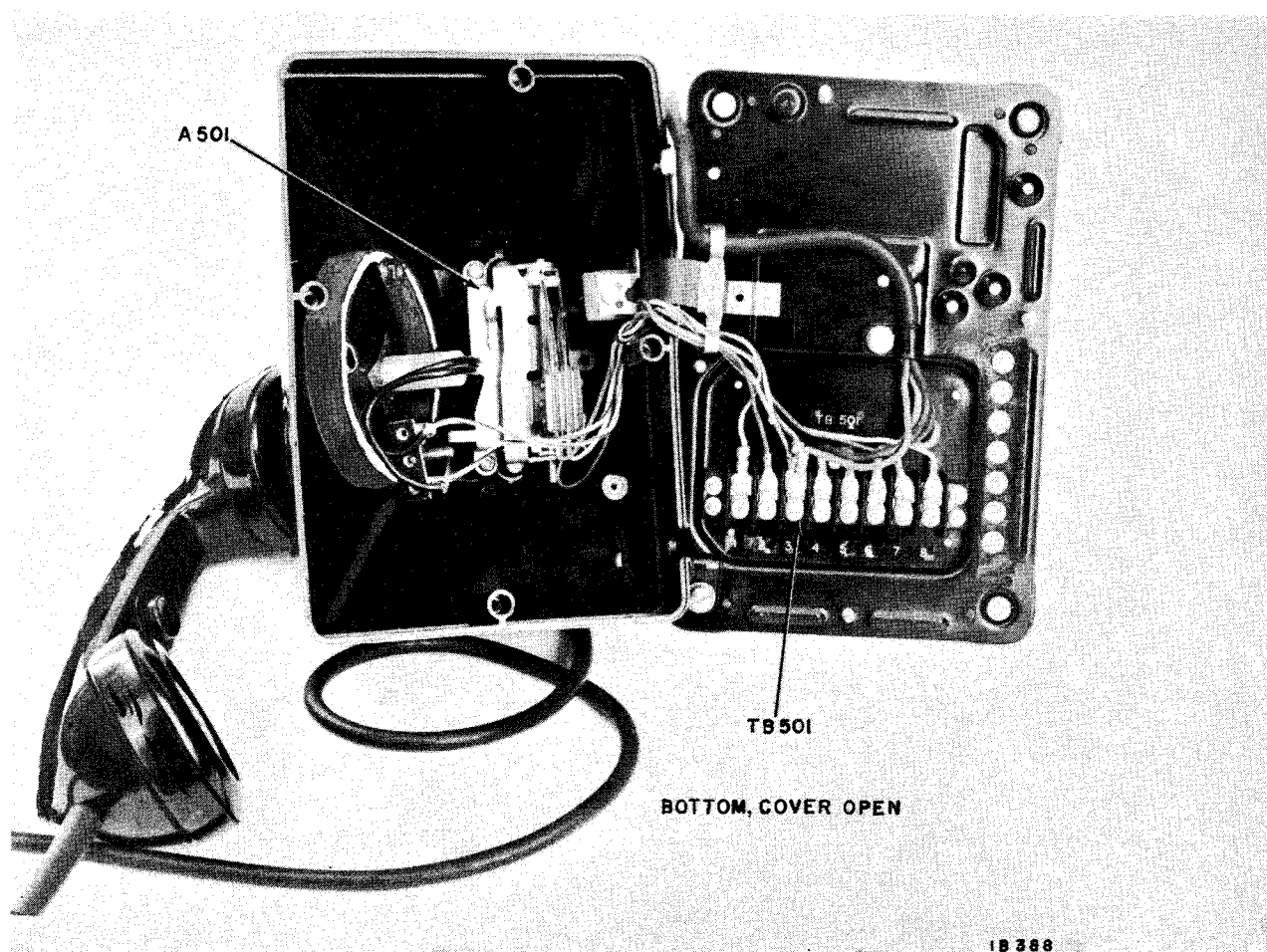
Figure 19. Remote Desk Set
