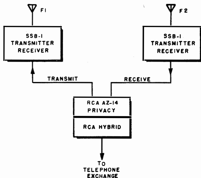
Figure 13. Duplex Radio Telephone Operation
