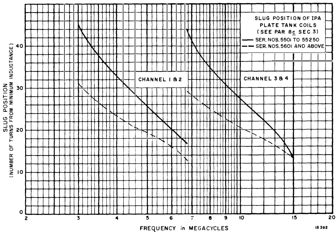
Figure 24. Slug Position of IPA Plate Tank Coils
