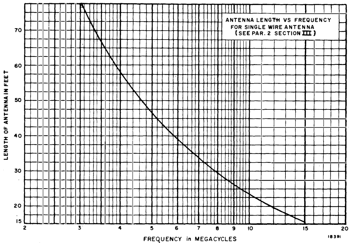
Figure 23. Antenna Length versus Frequency
