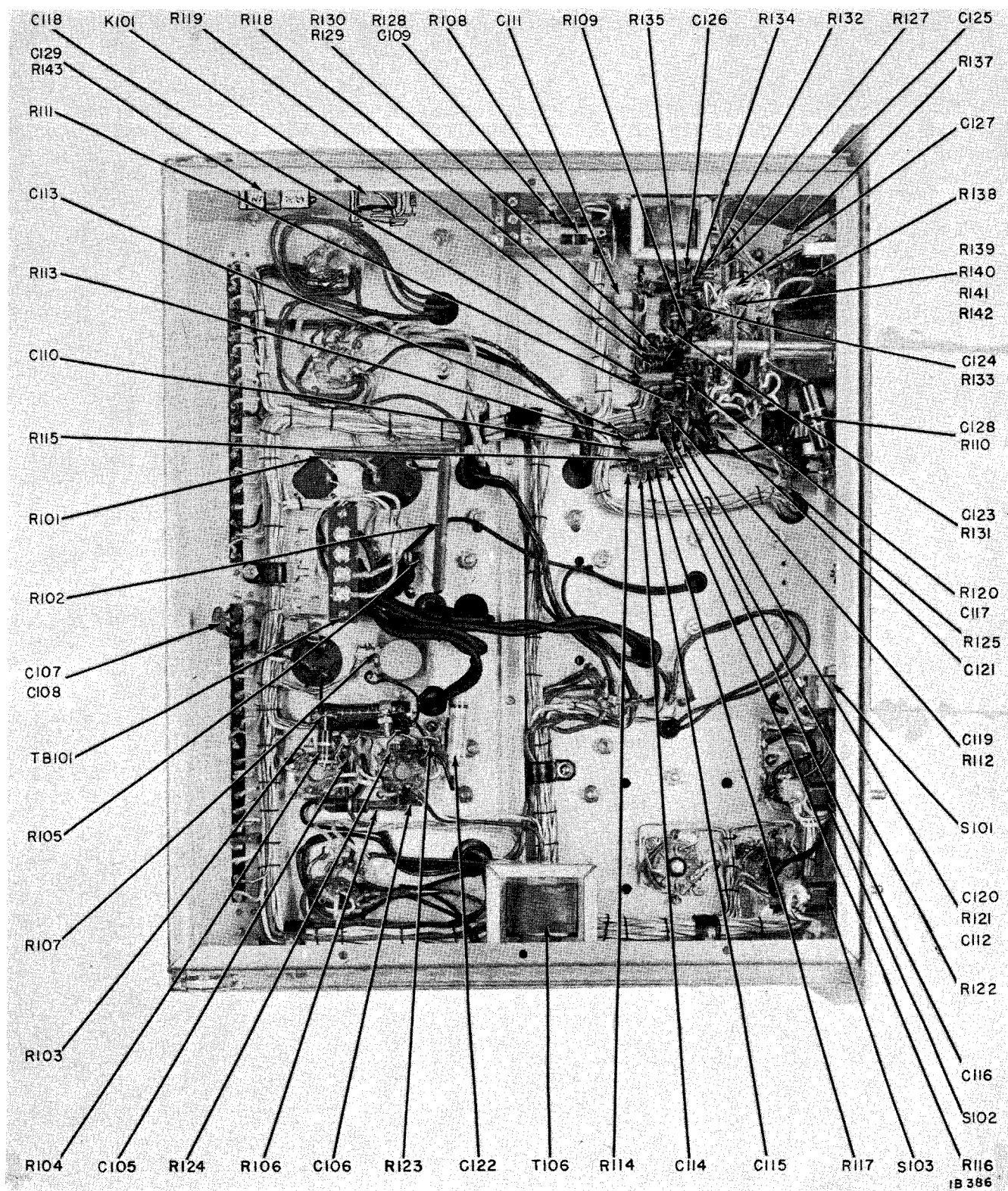
Figure 17. Power Supply, Bottom View
