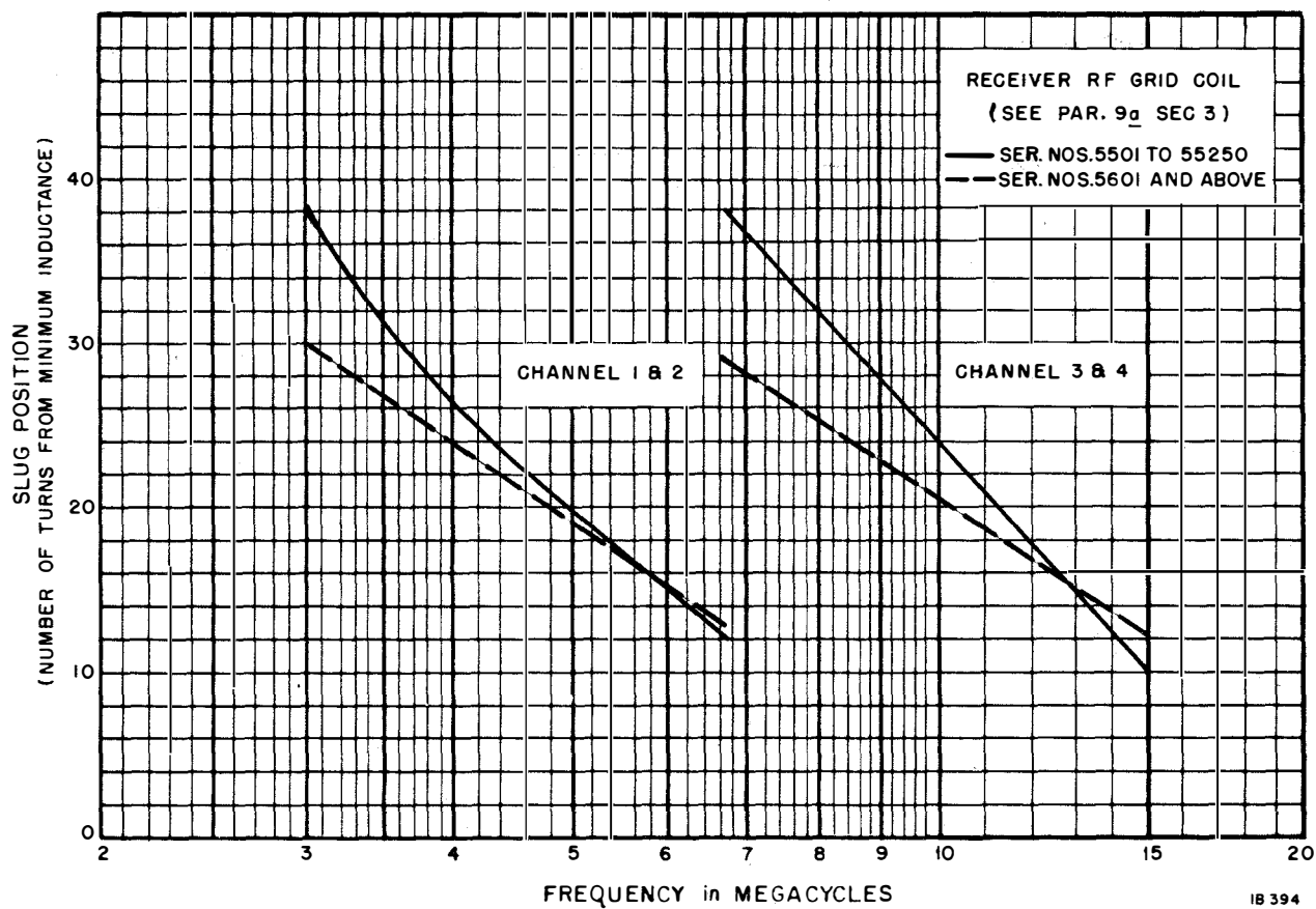
Figure 26. Slug Position of Receiver RF Coils
