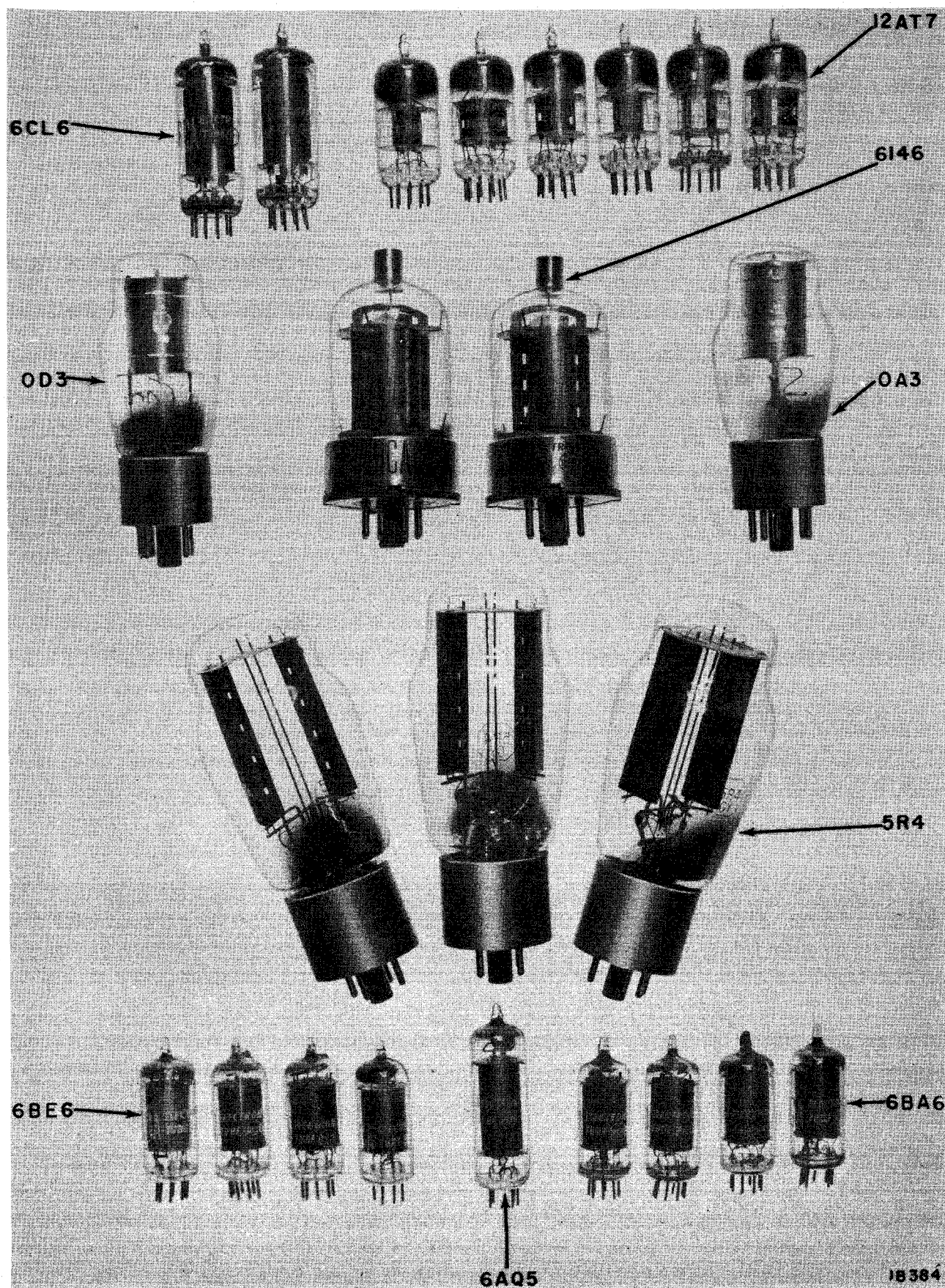
Figure 14. Tube Complement
