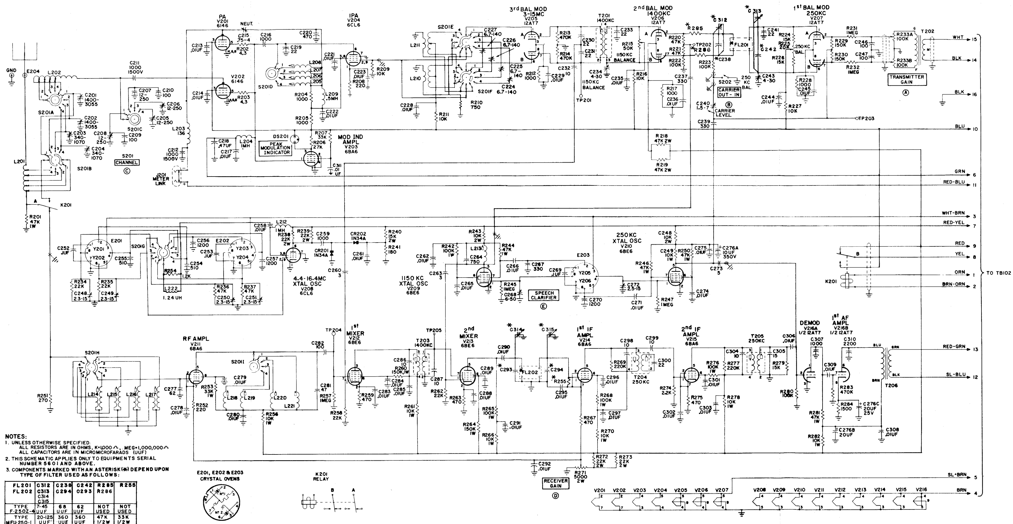
Figure 29B Transmitter-Receiver Schematic (Serial Numbers 5601 and above)
