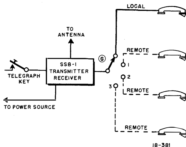
Figure 11. Simplex Radio Telephone Station
