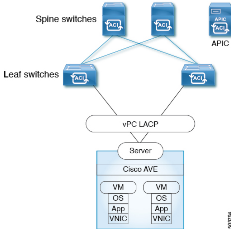
Figure 4: Direct Connection
