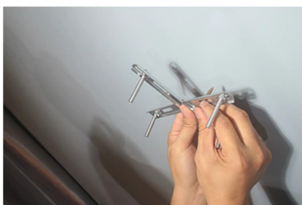
14: Install the cross with the sharp point screws to the ceiling, do not move the four flat headed screws
