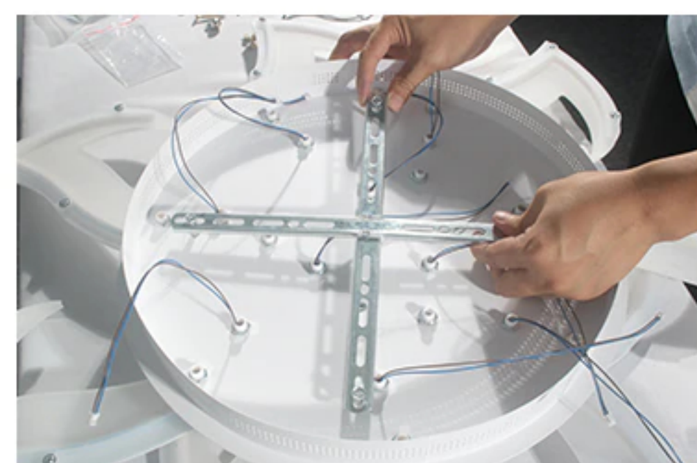
13: Put down the cross, find out the four small holes on the plate, make sure all the screws installed on the cross can go through the holes on the plate.
