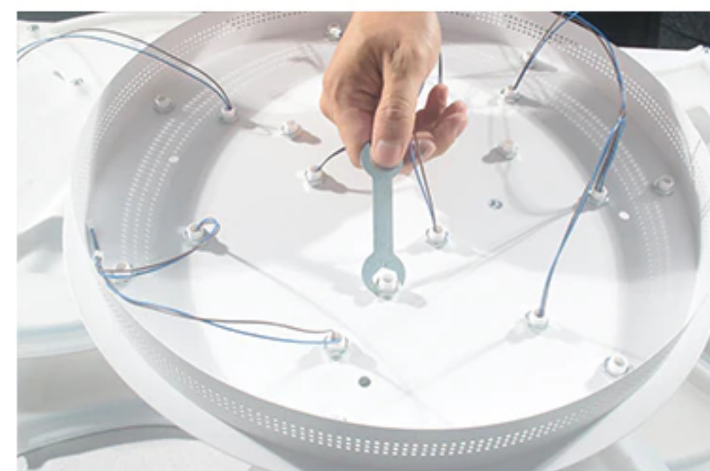
10: Use wrench to tight up the nuts further.
