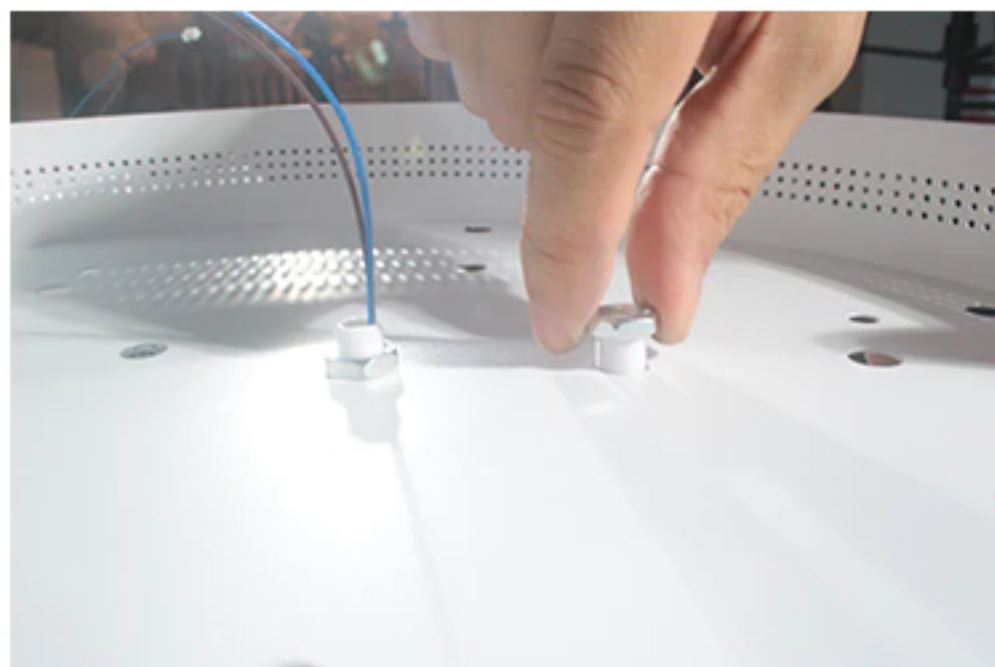
6: Fix the petals to the plate with nuts.
