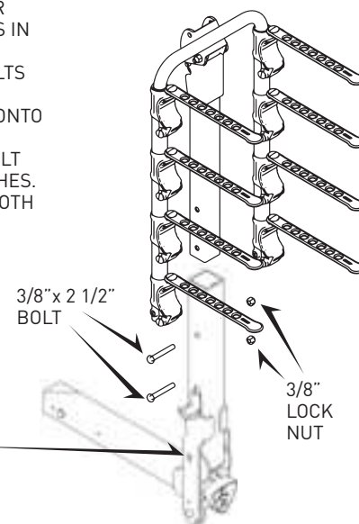
CARRY ARM ASSEMBLY
