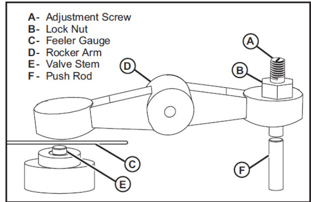
Figure 48 Set Valve Clearance
