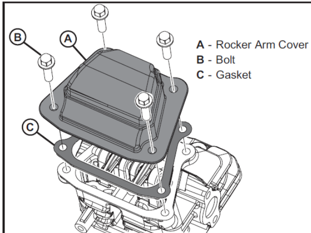
Figure 47 Remove Rocker Arm Cover
