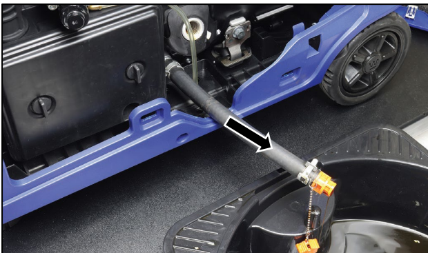
Figure 32 Draining the Engine Oil
