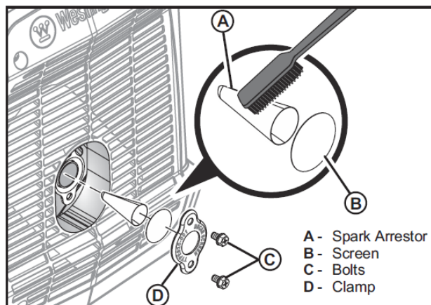
Figure 46 Remove and Clean the Spark Arrestor
