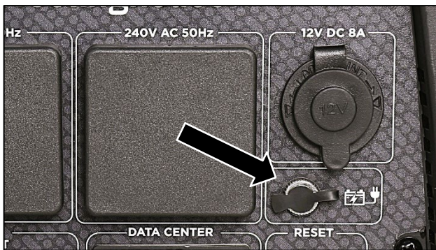
Figure 18 Connect the Battery Charger to the Generator
