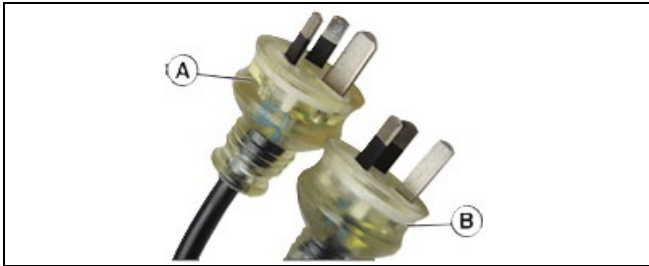
Figure 16 240-Volt AC Three-Pin Plugs
