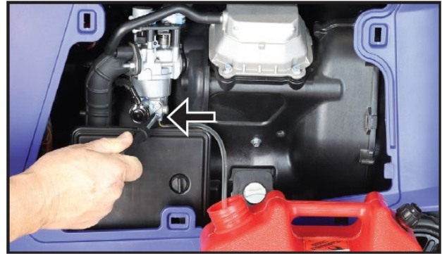
Figure 38 Drain the Carburettor
