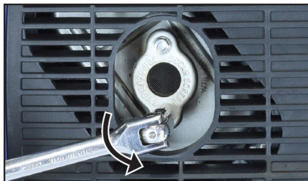
Figure 45 Remove the Spark Arrestor Clamp
