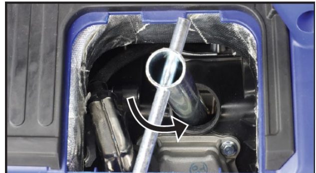
Figure 43 Remove the Spark Plug
