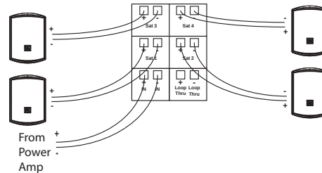
Using Four Control 52 Satellite Loudspeakers
