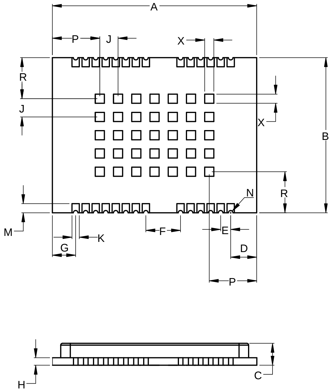
Figure 3-2 Mechanical Layout
