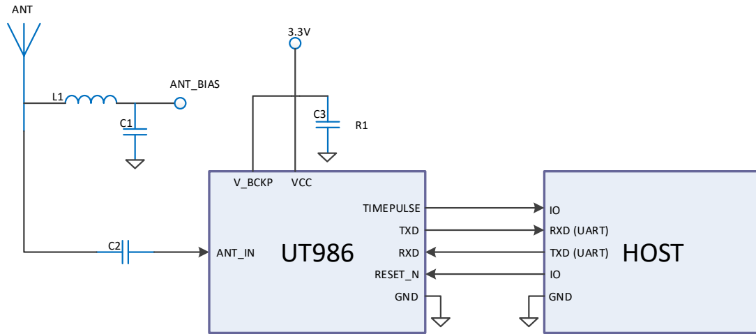
Figure4-1 UT986 Minimal Design
