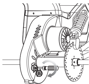
8 Position the chain guard to align mounting holes and, using a Phillips screwdriver, screw to frame.
