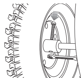
10 On the inside of the wheel slide bolt through wheel and axle and, using a 5 mm Allen wrench and a 10 mm wrench, secure with nut.
