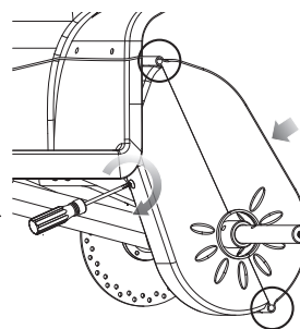
9 Position the chain guard to align mounting holes and, using a Phillips screwdriver, screw to frame.
