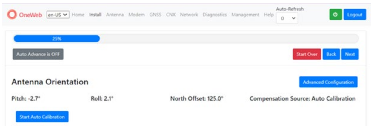
Figure 92: LUI – Antenna Orientation - Auto Calibration
