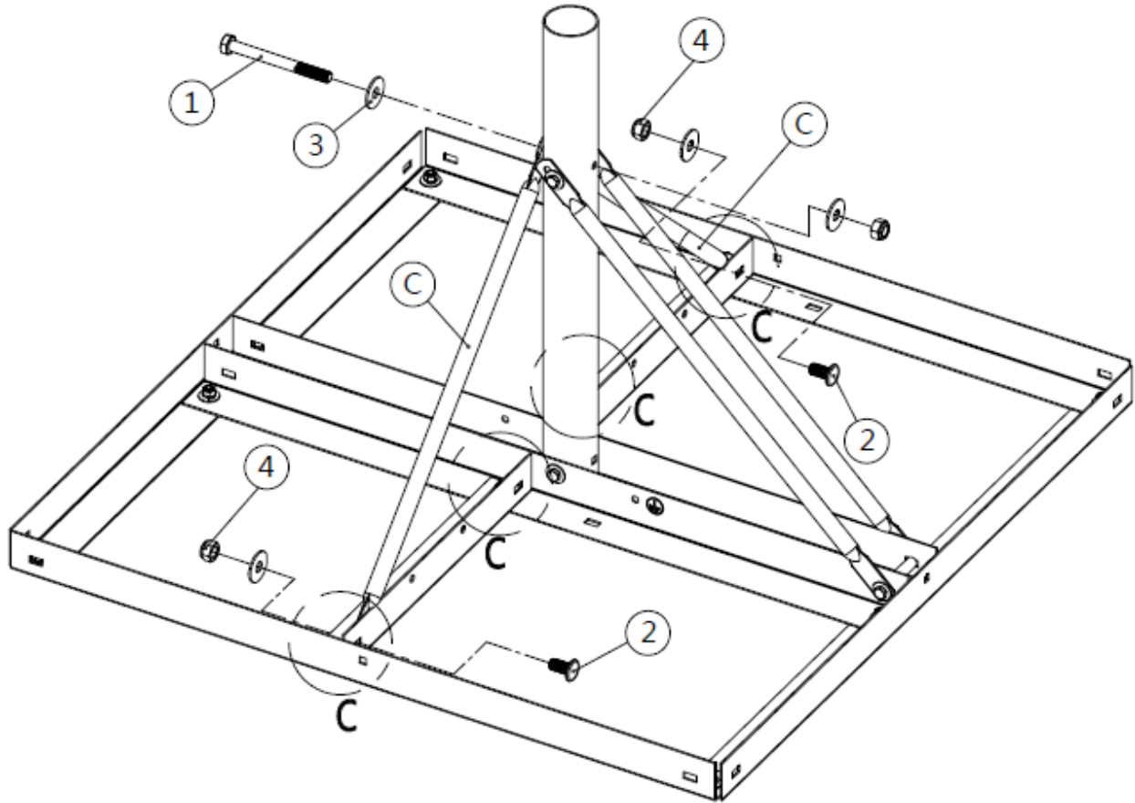
Figure 28: Installing the second two side supporting rods
