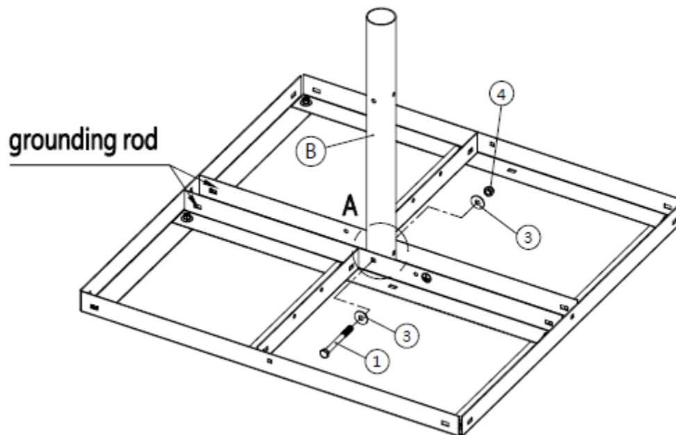
Figure 25: Installing the mast pole
