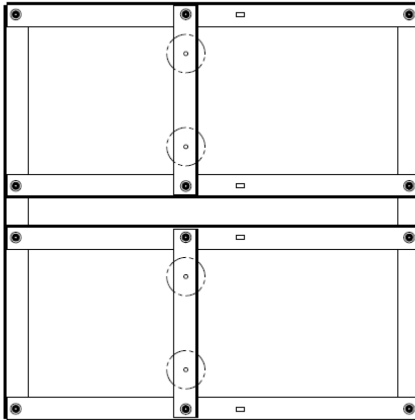
Figure 31: Penetrating fastener mount locations
