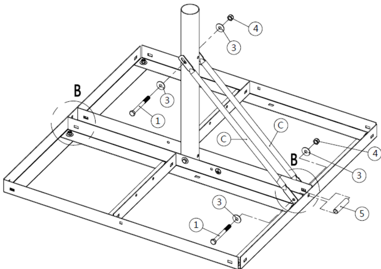
Figure 27: Installing the first two side supporting rods
