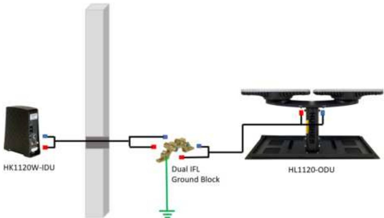
Figure 35: Hughes AAA UT IFL routing
