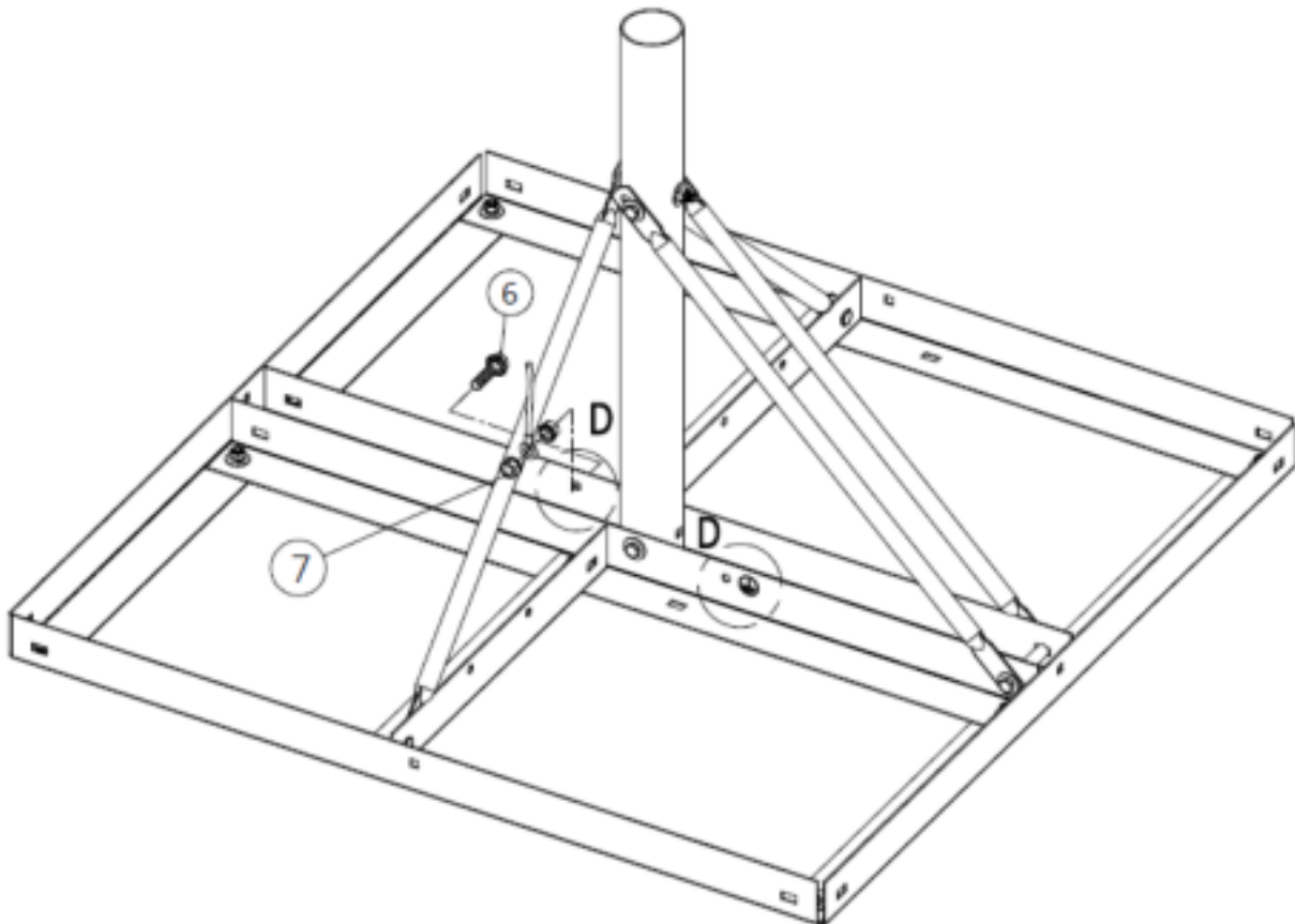
Figure 30: Installing the grounding cable
