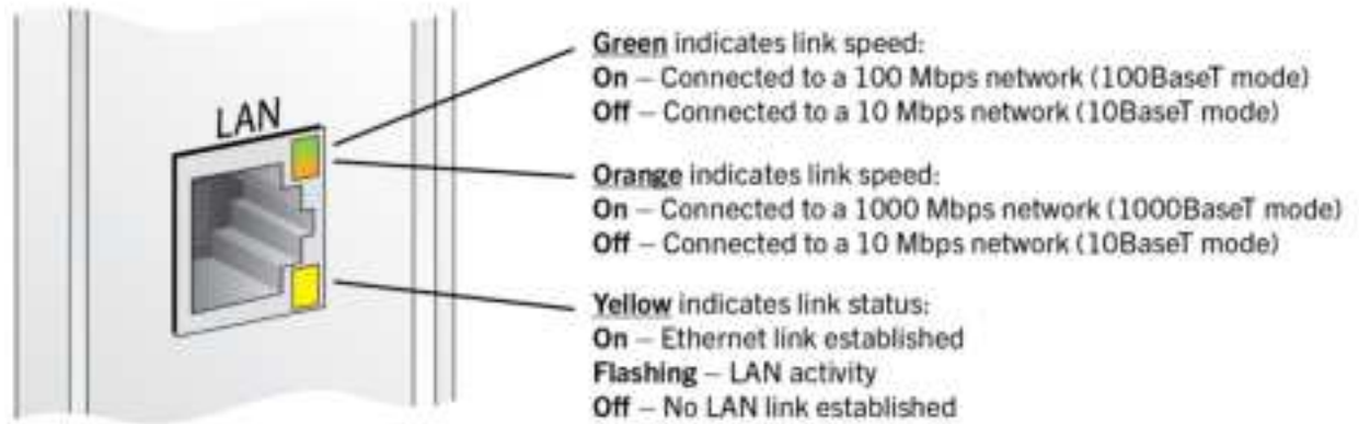
Figure 110: LAN port LEDs
