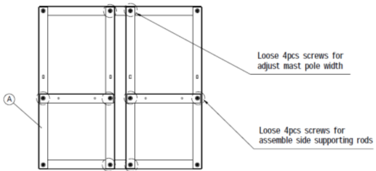
Figure 24: Loosening the ground mounting screws
