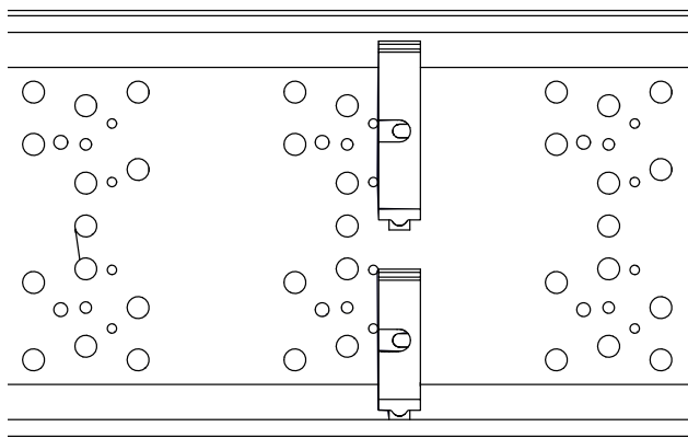
Fig. 68: 7-pole hanger clamp 0831
