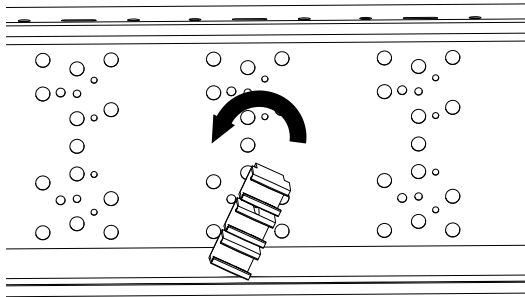
Fig. 28: Hook 3-pole hanger clamp onto ProShell 206 Support Profile System
