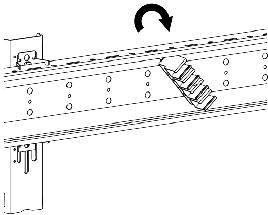
Fig. 22: Turn hanger clamp 0812 onto ProShell support profile rail
