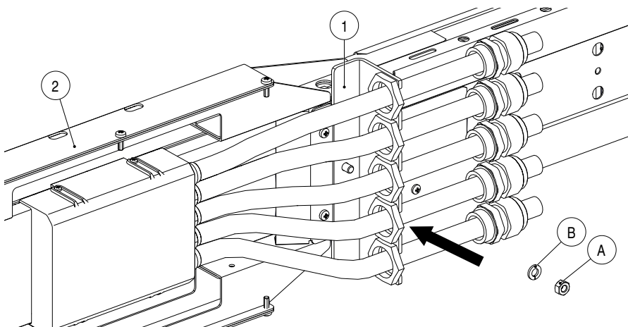
Fig. 75: Install strain relief plate (1)
