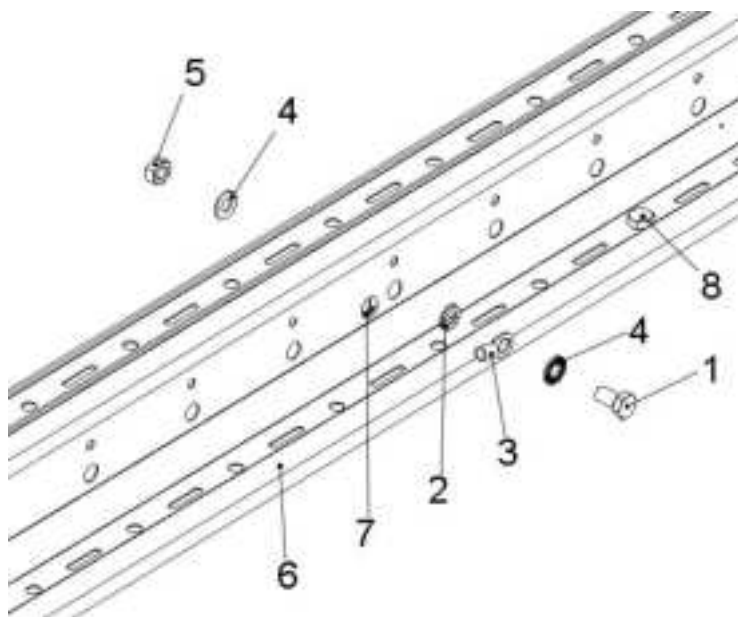
Fig. 55: Installation of PE cable on support profile (exploded view)
