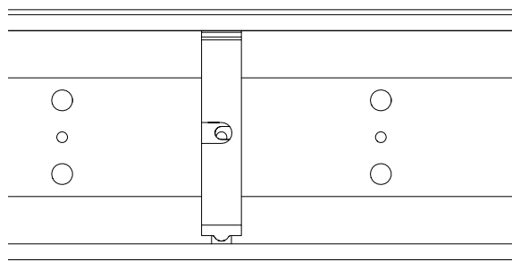
Fig. 62: Install hanger clamp 0831 onto ProShell support profile rail
