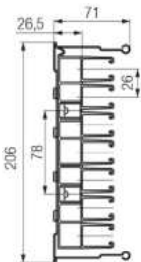
Fig. 26: Dimensions of 7-pole hanger clamp 0812
