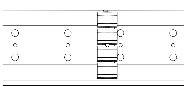
Fig. 23: Install hanger clamp 0812 onto ProShell support profile rail 128
