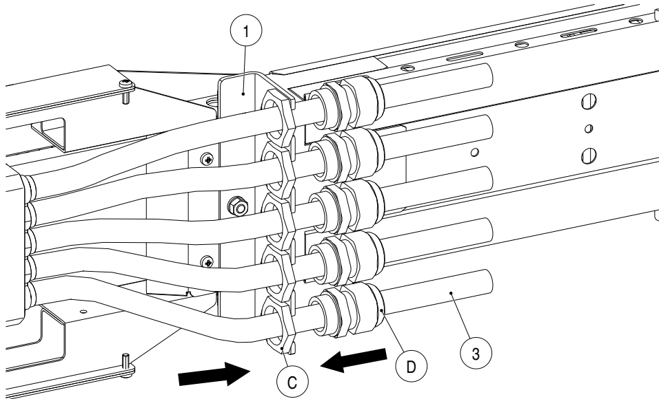
Fig. 76: Screw connecting cables (3) to strain relief plate (1)
