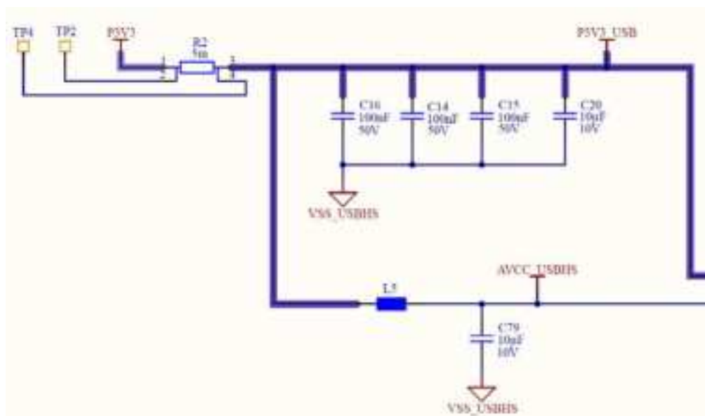
Figure 34. RA USB Current Measurement Circuit
