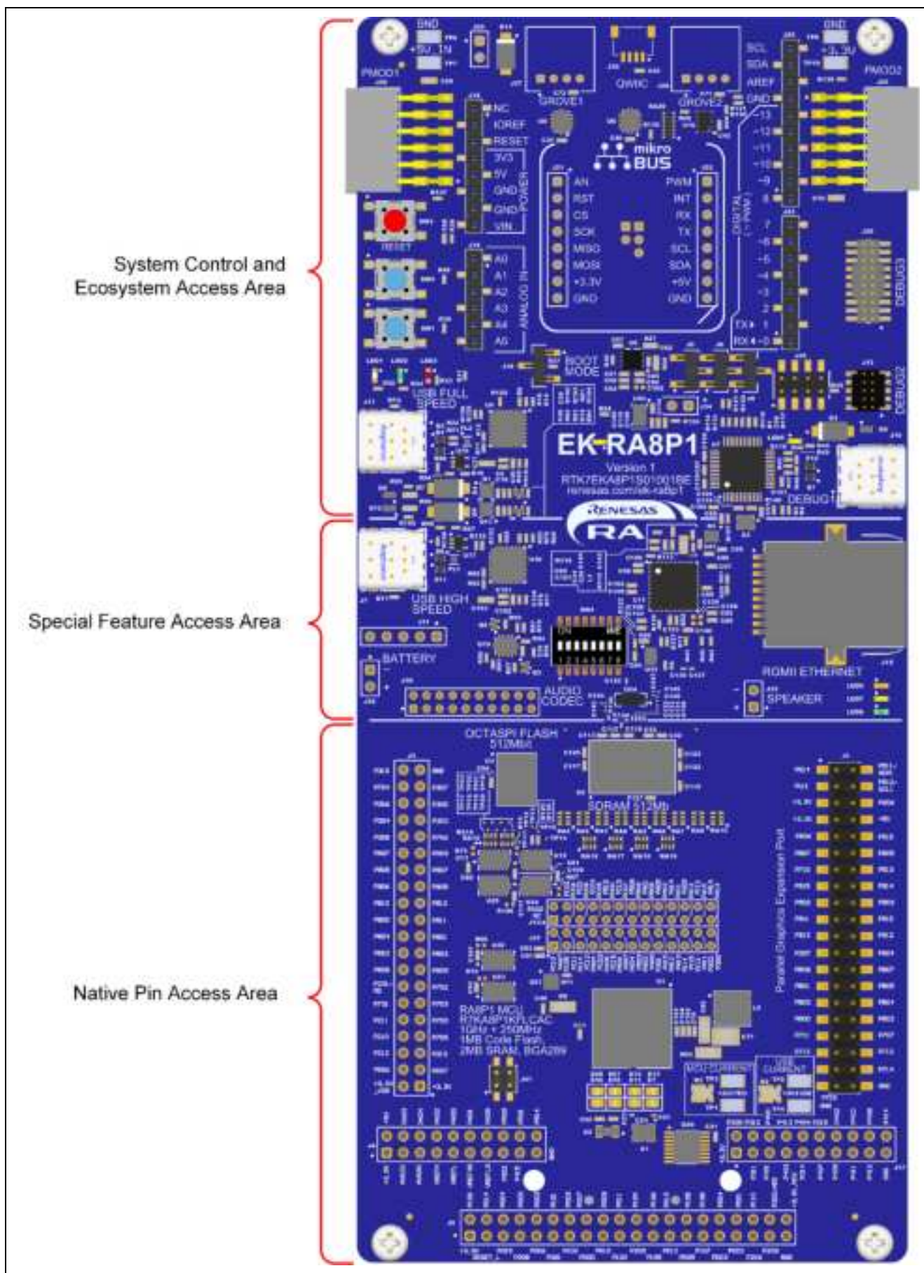
Figure 4. EK-RA8P1 Board Functional Area Definitions
