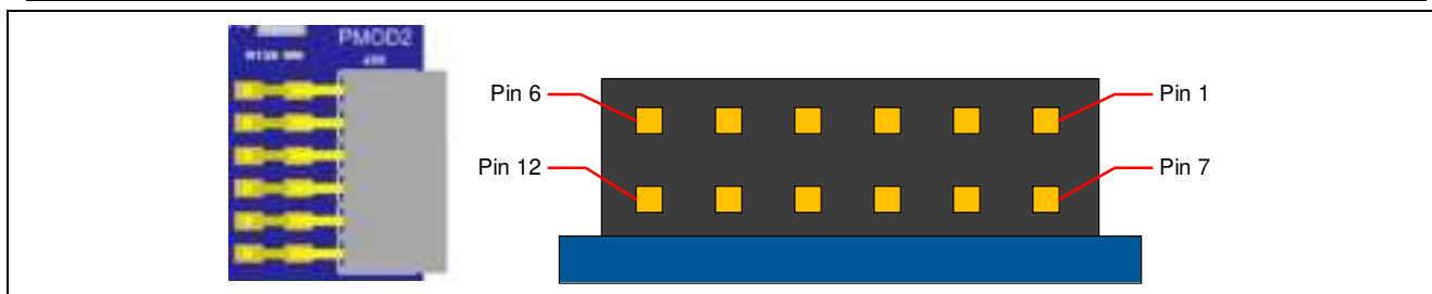
Figure 14. Pmod 2 Connector
