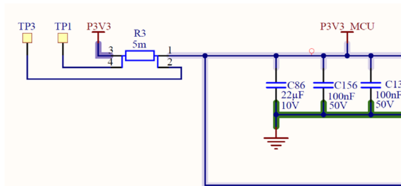
Figure 35. RA +3.3 V Current Measurement Circuit
