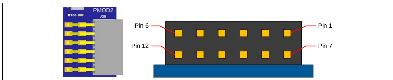
Figure 14. Pmod 2 Connector
