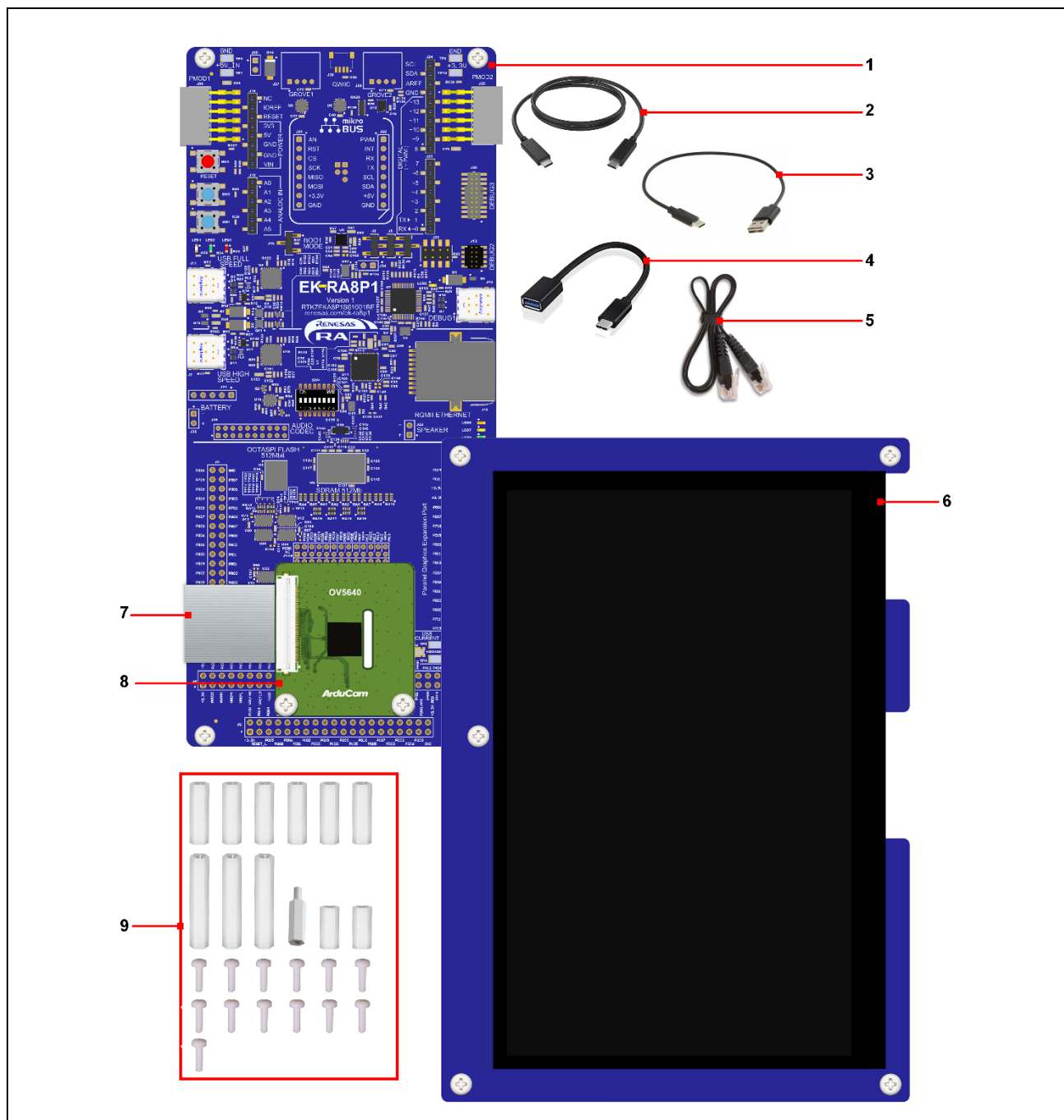
Figure 3. EK-RA8P1 Kit Contents
