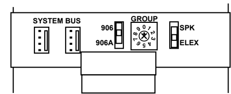
Figure 34. 906 Control Panel connections and settings.
