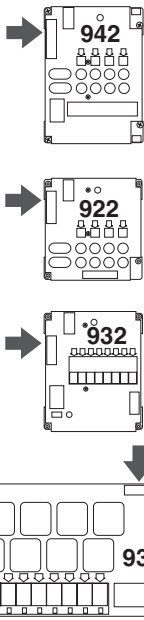
Figure 14. Main Switching Modules and location of Group switch. (Model 910D is always Group 0.)
