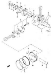
FIG.7 CRANKSHAFT (C-3)
