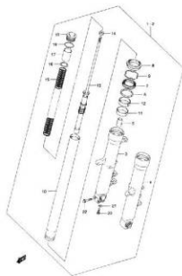
FIG.54 FRONT DAMPER (MODEL K2) (J-6)
