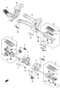
FIG.37 FOOTREST (H-4)
