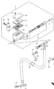
FIG.60 CLUTCH MASTER CYLINDER (J-13)
