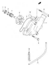
FIG.18 WATER PUMP (D-9)
