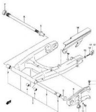
FIG.61 REAR SWINGING ARM (K-2)
