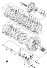
FIG.22 CLUTCH (E-2)
