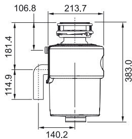
FRAGMENTA FWD 75 S TECH 3/4 HP
