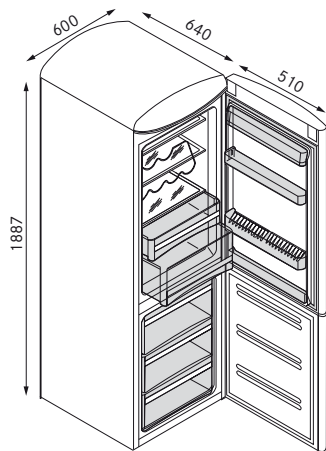
COMBI NEW VINTAGE
