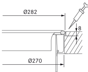
WASTE-BIN FLUSH-M F12
