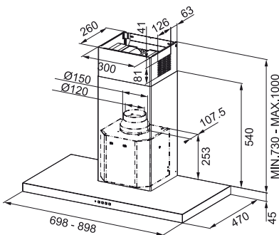
FLAT EB 70 FLAT EB 90
