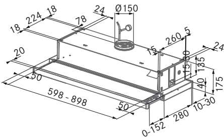
TELESCOPICA 60 CS 262 TELESCOPICA 90 3 GAX 90
