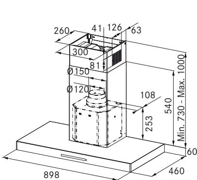
CRYSTAL TOUCH 90 / CRYSTAL EB 90
