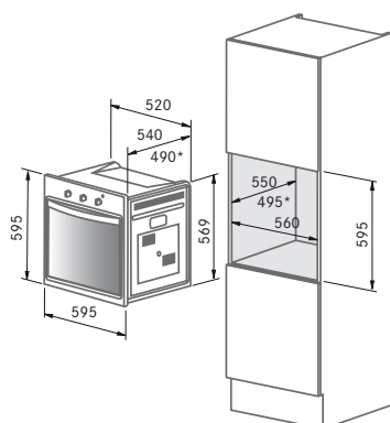
CRYSTAL PYRO 60 CRYSTAL DCT 60 CRYSTAL 60
