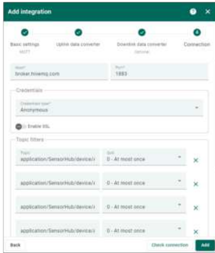
Figure 104: Configure the connection options
