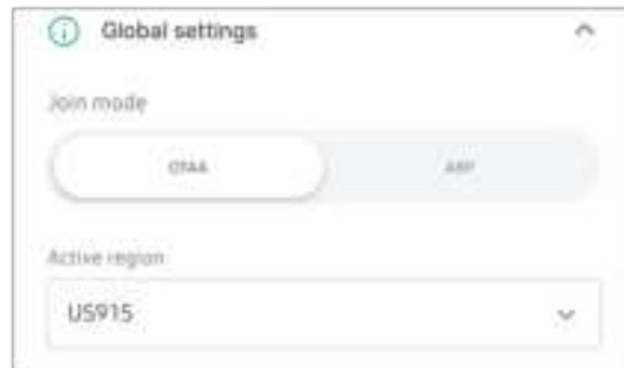
Figure 35: Global Settings
