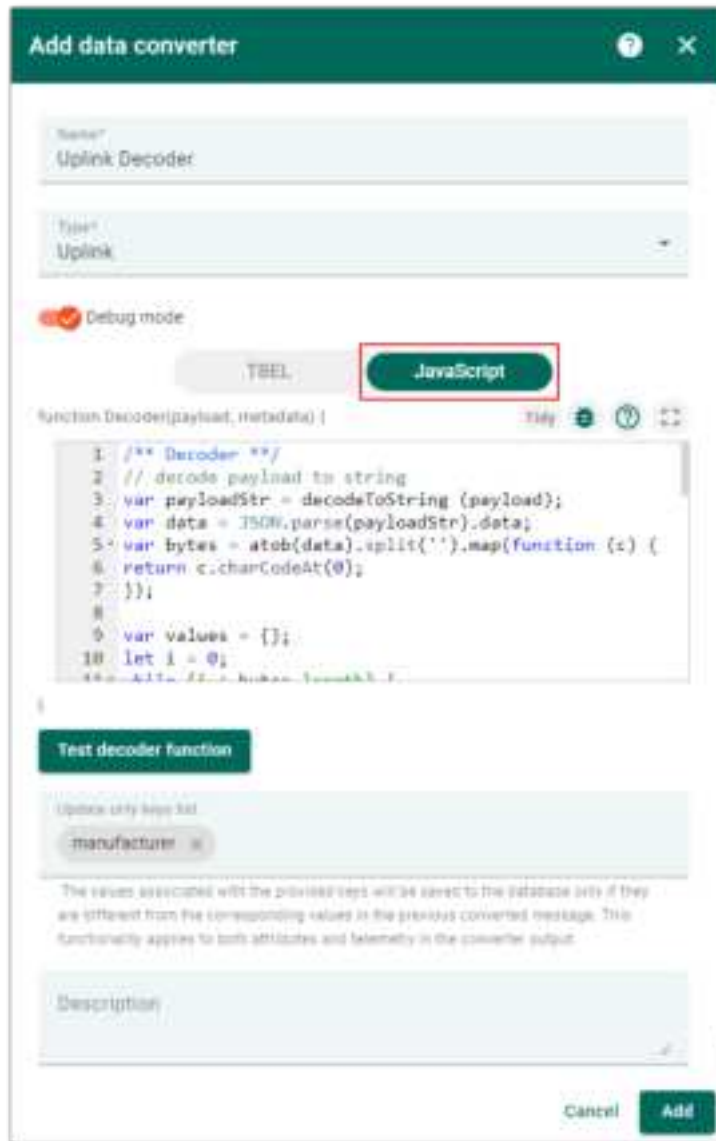
Figure 100: Add the decoder code
