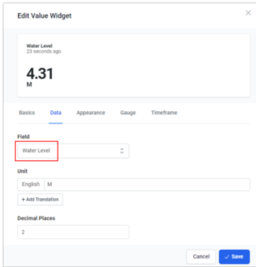
Figure 146: Select the visualization data field
