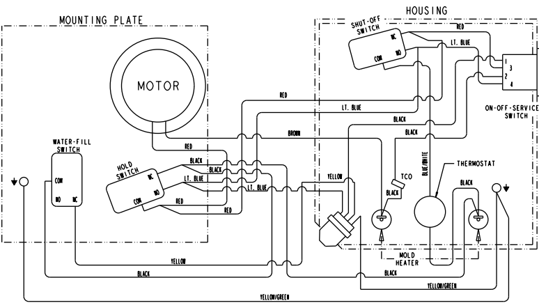
WIRING DIAGRAM SERVICE START FEATURE
