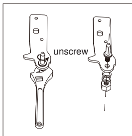
Step 6: Unscrew and remove the bottom hinge pin, turn the bracket over and replace it.
