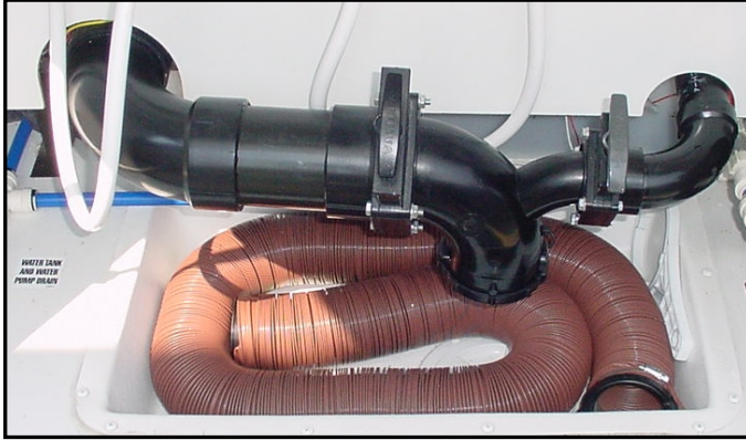
Figure 11-13. Sewer Hose and Drain Connections
