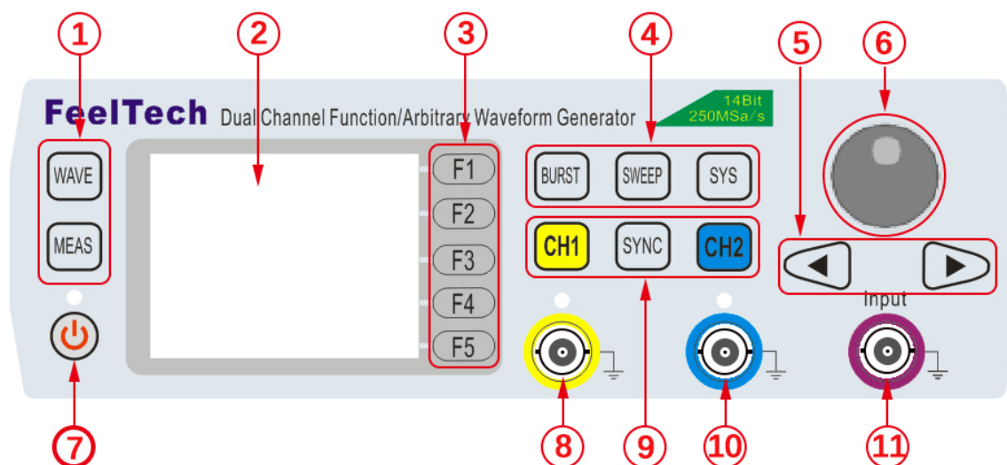
Front Panel
