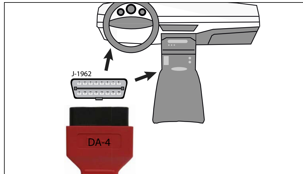
Figure 4-4 DA-4 data cable (16-pin end) connection to vehicle DLC (typical DLC locations)
